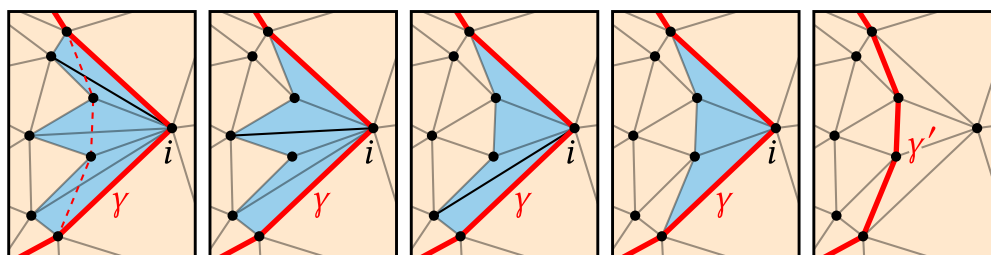
Fig. 33. FLIPOUT shortens the curve \gamma by repeatedly flipping edges to introduce a shorter path.
