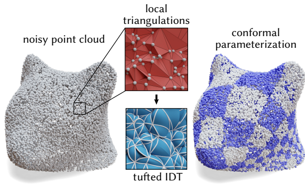
Fig. 42. The tufted intrinsic Delaunay point cloud Laplacian, demonstrated here for spectral conformal parameterization of a point cloud [Mullen et al. 2008].
