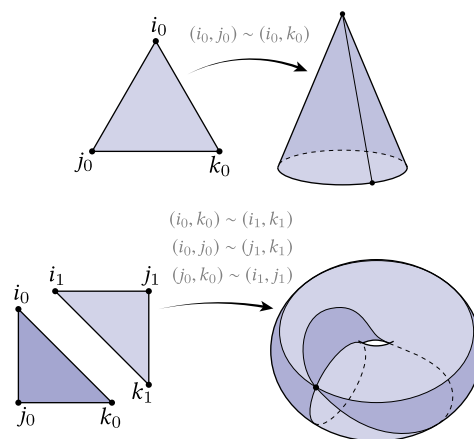
Fig. 8. In a \Delta -complex, the vertices of an edge or triangle are not required to be distinct. For instance, one can build a cone by gluing together two edges of the same triangle (top), or a torus out of two triangles and just a single vertex (bottom).
