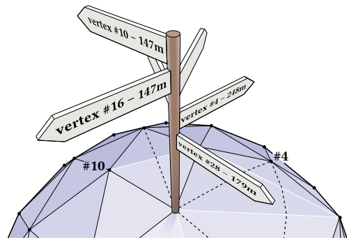
Fig. 20. Signposts encode edges of an intrinsic by storing the length and direction of each edge in the tangent space each vertex.
