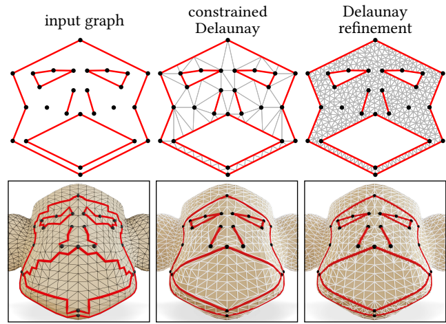
Fig. 25. Top. Planar constrained Delaunay triangulations are used to produce high-quality triangulations which conform to a collection of specified lines. Bottom. Constrained intrinsic triangulations play a similar role on surfaces, preserving a set of intrinsic edges in the triangulation.
