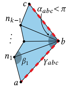
Fig. 34. Notation for FLIPOUT.
