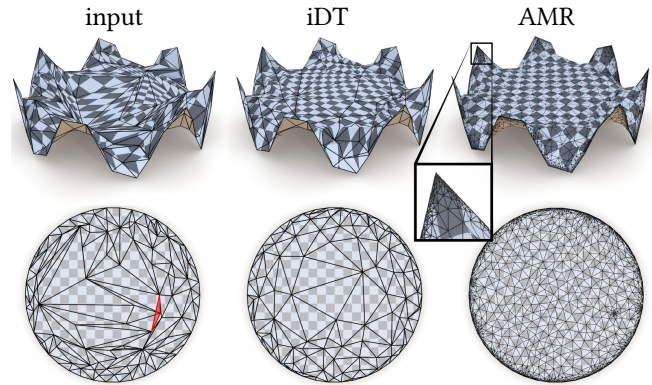
Fig. 30. Using an intrinsic Delaunay triangulation ensures that a harmonic parameterization is flip-free, while adaptive mesh refinement provides high-resolution in the interesting regions of the mesh. [Sharp et al. 2019b]
