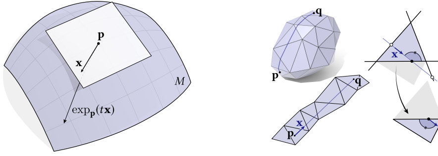
Fig. 17. Left : the exponential map simply walks along the surface in a given direction \mathbf{x} , starting at a given point \mathbf{p} . Right : on a triangle mesh, the exponential map can be computed by tracing out a straight line through a strip of triangles. Each step amounts to performing ray-edge intersections, then transporting the ray direction vector to the next triangle.
