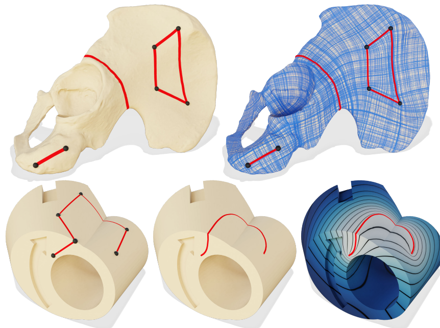
Fig. 40. PDEs taking boundary conditions from constrained intrinsic triangulations. Top , a cross field conforming to curves on a 3D scan of a pelvis [Knöppel et al. 2013], and bottom , a Poisson equation with boundary conditions defined along a Bézier curve on a mechanical part.
