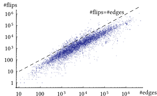
Fig. 23. An empirical study of the number of edge flips to produce an intrinsic Delaunay triangulation [Sharp et al. 2019b]. Each point is a 3D model from the Thingi10k dataset [Zhou and Jacobson 2016]. The observed complexity trend is linear, even on these difficult models.
