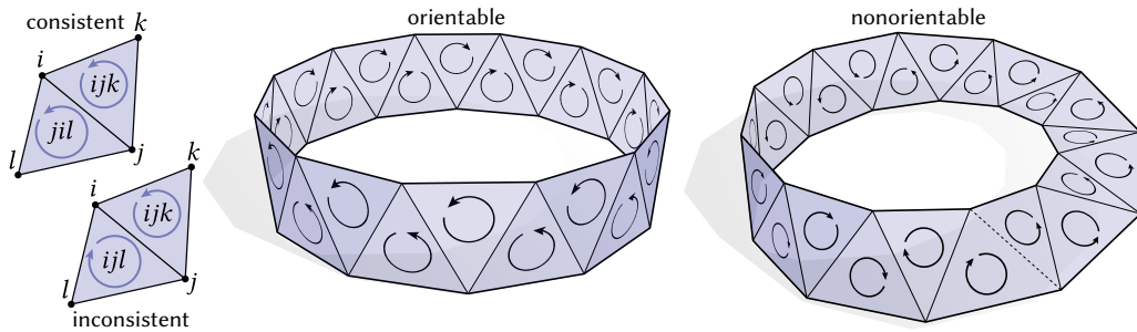
Fig. 6. Left : a pair of triangles is consistently oriented if they disagree on the orientation of the shared edge. A triangulation is orientable if all triangles can be assigned consistent orientations ( center ) and nonorientable otherwise ( right ).
