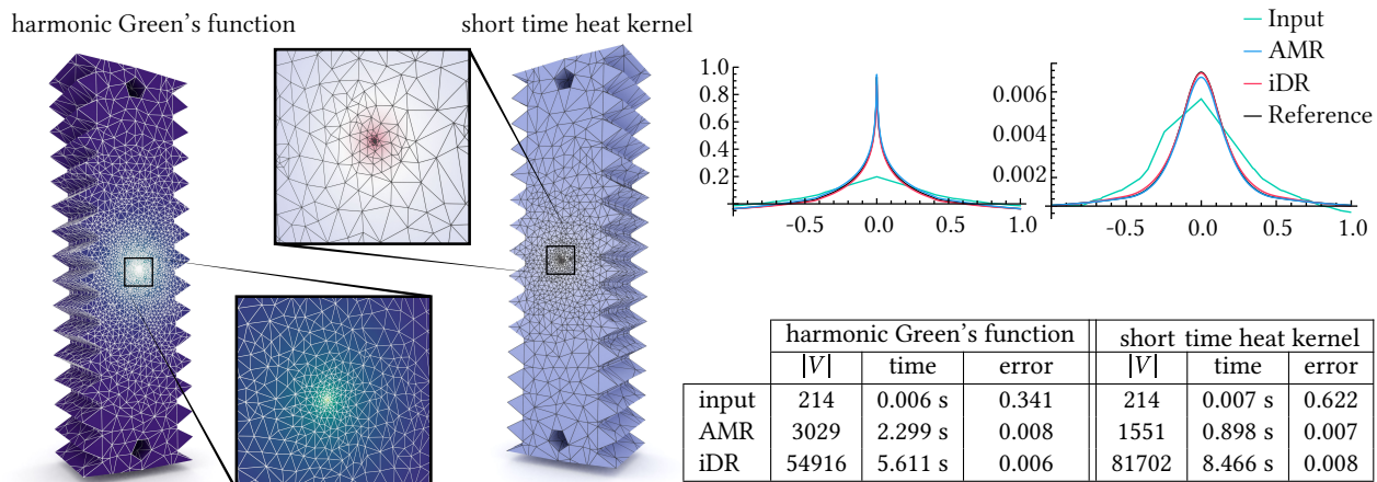
Fig. 26. Intrinsic AMR allows one to efficiently compute standard geometric kernels to high accuracy. Performing ordinary Delaunay refinement to the same accuracy requires 18x and 54x as many vertices on the harmonic Green's function and short time heat kernel resp. [Sharp et al. 2019b].
