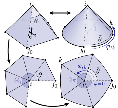
Fig. 14. Local coordinate system for tangent vectors at vertices.
