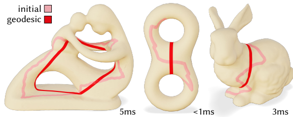
Fig. 38. Geodesic loops generated by with edge flips in an intrinsic triangulations. Inset values give the runtimes.
