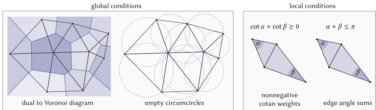
Fig. 22. There are many equivalent characterizations of the Delaunay triangulation. Here we illustrate a few examples.
