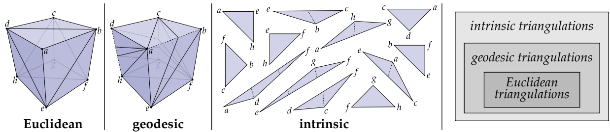
Fig. 2. Traditionally, mesh edges are straight line segments in Euclidean space (far left). The much larger spaces of geodesic and intrinsic triangulations provide tremendous additional flexibility by allowing edges to be straight paths along the surface (center left), or by just considering an abstract collection of triangles identified along shared edges (center right).
