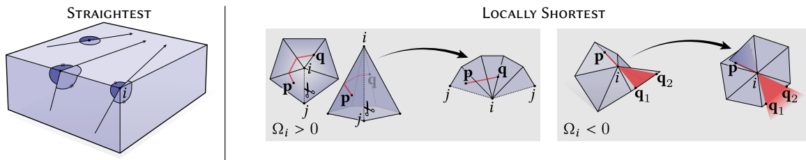
Fig. 16. There are two distinct ways to define geodesics on polyhedra: as “straightest” curves, with equal angle on both sides ( left ), or as “locally shortest” curves that cannot be pulled tighter ( right ). A curve through a positively-curved vertex ( \Omega_i > 0 ) can always be made shorter, whereas there are many ways to continue a path through a negatively-curved vertex ( \Omega_i < 0 ) while remaining locally shortest—for example, a path from p through i and then to either q_1 or q_2 is locally shortest. For intrinsic triangulations, we need only consider locally shortest geodesics. ( Leftmost figure adapted from [Polthier and Schmiees 2006] )
