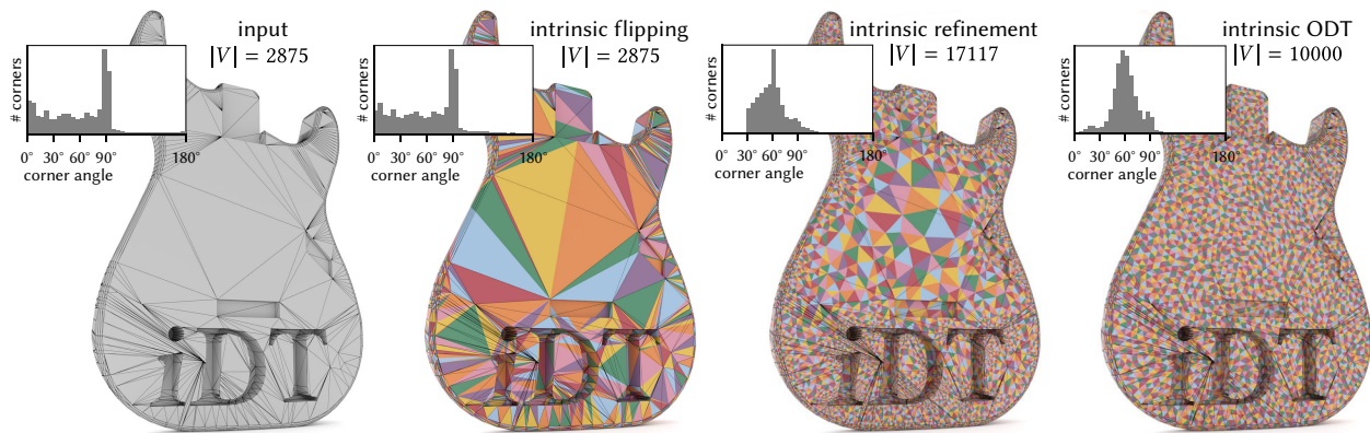
Fig. 21. Intrinsic retriangulation schemes applied to a computed-aided design model with poor triangle quality. The black wireframe denotes the extrinsic mesh, colored triangles give the intrinsic triangulation. Delaunay flips achieve the Delaunay property for a fixed vertex set, while refinement and repositioning further improve triangle quality and vertex distribution.
