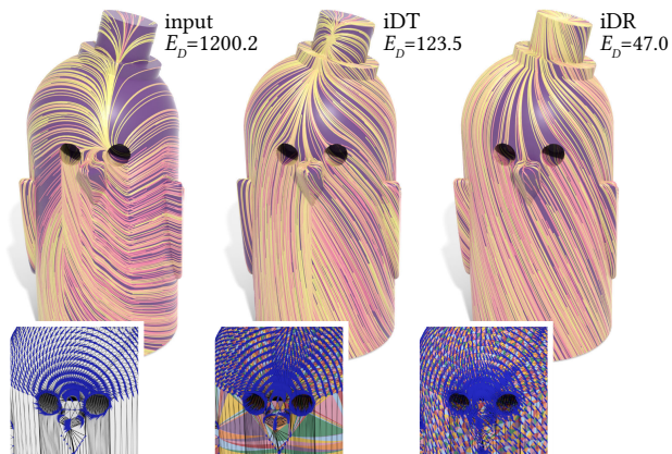
Fig. 32. The signpost data structure also enables processing tangent data. Here, smoothest vector fields computed on an intrinsic triangulation have much lower Dirichlet energy than one computed on a low-quality mesh. [Sharp et al. 2019b]
