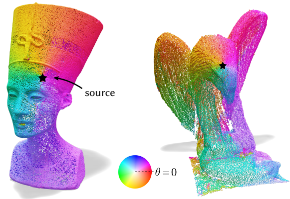
Fig. 43. Angular parameterizations of point clouds, computed with the tufted intrinsic Delaunay point cloud Laplacian via the vector heat method [Sharp et al. 2019c].
