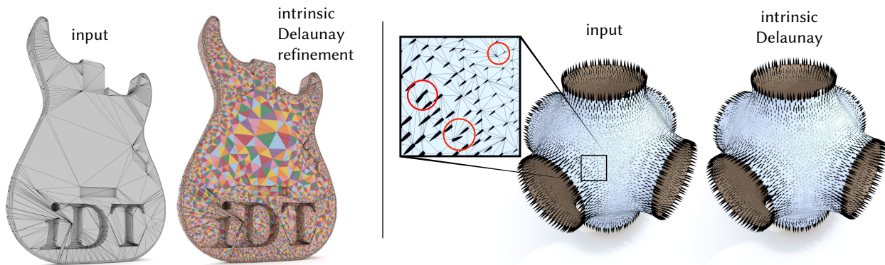
Fig. 24. Left : Rich data structures enable intrinsic Delaunay refinement, generating triangulations with good angle bounds. The black wireframe denotes the extrinsic mesh, while colored triangles give the intrinsic triangulation. Right : Signposts further enable vector field processing; the Laplacian of the intrinsic Delaunay triangulation offers a maximum principle for tangent vector fields, which here avoids unexpected flipped vectors when generating a smooth field.
