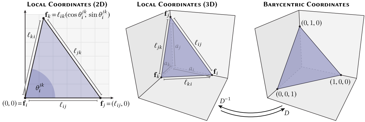
Fig. 13. Given the three edge lengths of a triangle \ell_{ij}, \ell_{jk}, \ell_{ki} , one can find a corresponding set of vertex positions \mathbf{f}_i, \mathbf{f}_j, \mathbf{f}_k in either 2D (left) or 3D. For acute triangles, one can construct a 3D embedding where the vertices lie along the coordinate axes (middle), which is related to the barycentric coordinates by a simple diagonal scaling D (right). The same strategy can be generalized to obtuse triangles via a complex-valued embedding.
