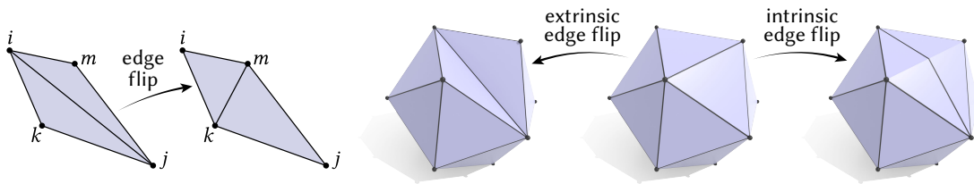
Fig. 11. Left : an edge flip modifies the connectivity of a triangle mesh, replacing triangles ijk, jim with triangles kmi, mkj . Right : whereas an ordinary extrinsic edge flip changes the mesh geometry, an intrinsic flip leaves the original geometry untouched.
