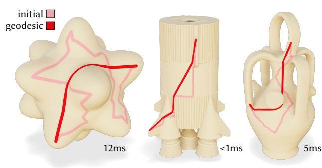
Fig. 35. Basic results shortening an initial path to a geodesic by flipping edges. Inset values give the runtimes. All of the resulting curves shown are exact polyhedral geodesics.
