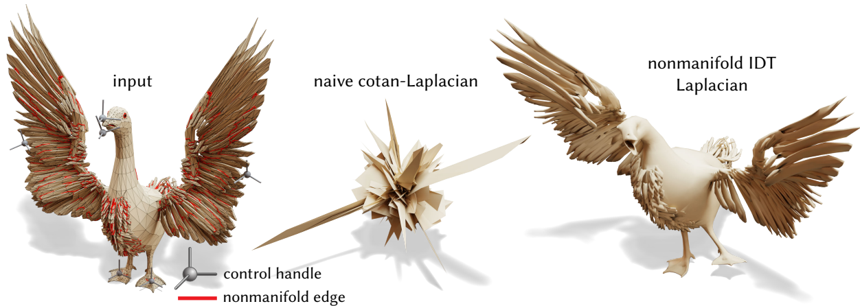
Fig. 41. Robustness in the context of differential surface editing [Lipman et al. 2004; Sorkine et al. 2004; Yu et al. 2004], where a system of equations involving a Laplacian is solved to deform a 3D model. Applying these techniques naively in the extrinsic mesh, which is nonmanifold and has many low-quality triangles, yields only numerical noise. Substituting the nonmanifold IDT Laplacian constructed on the tufted cover generates the expected smooth deformation.
