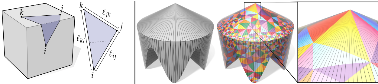
Fig. 3. Conceptually, intrinsic triangles can “bend” across an underlying polyhedron, yet still flatten out into standard triangles described by three ordinary edge lengths (left). This flexibility enables things that are impossible with standard, extrinsic algorithms—here, a mesh with tiny input angles becomes a geometrically identical Delaunay triangulation with angles no smaller than 30^\circ (right). Since the output is described by conventional data (connectivity + edge lengths) it can still be used directly by many standard simulation and mesh processing algorithms.
