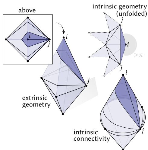
Fig. 7. Intrinsic triangles can “wrap around” extrinsic polyhedra, allowing them to have unusual connectivity. Here, for instance, the dark blue triangle connects once to vertex i and twice to vertex j —effectively gluing two of its sides to each other along edge ij .
