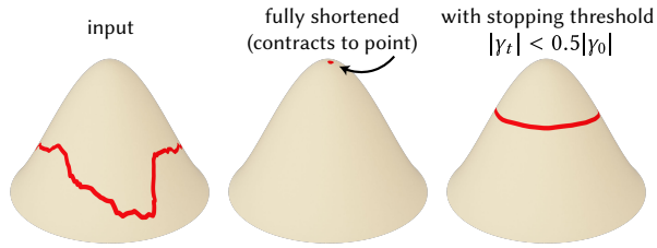
Fig. 37. Algorithm 7 acts as discrete curve-shortening flow; stopping the procedure early via a length or angle threshold generates straighter curves, without drifting too far from the initialization or contracting to a point.
