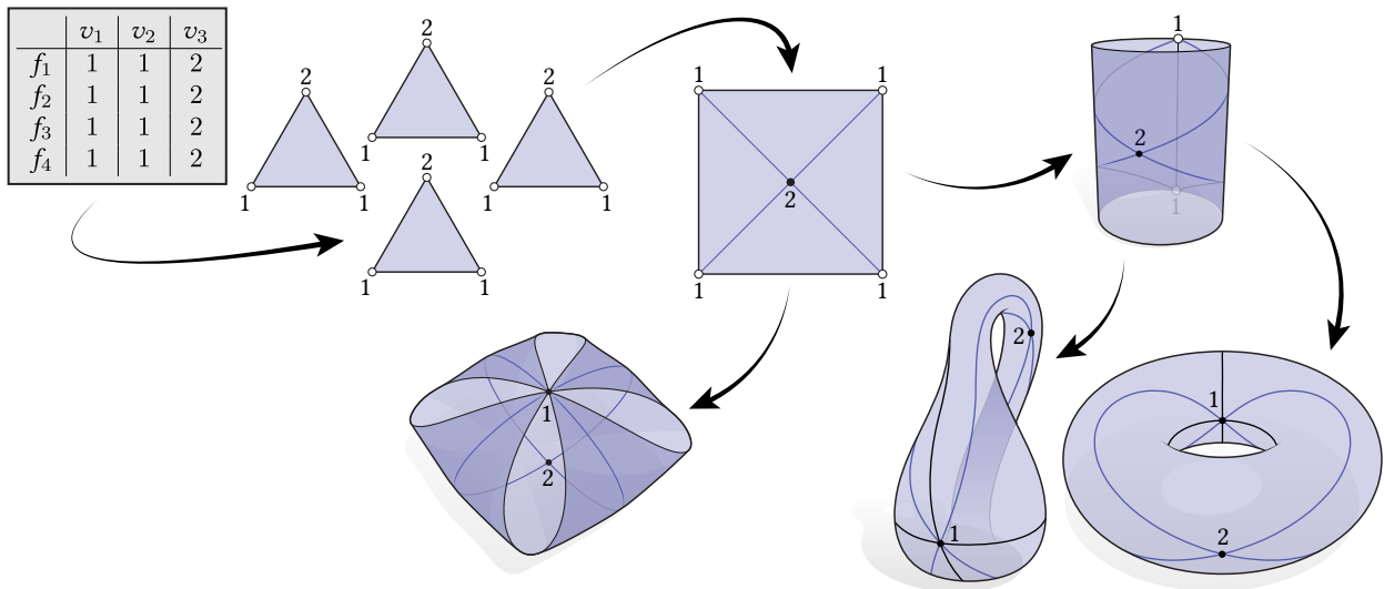
Fig. 9. A basic vertex-face adjacency list (top left) provides an ambiguous encoding of connectivity. Here, for instance, it specifies that the mesh is comprised of four triangles and two distinct vertices. However, without additional information about how edges are glued together, there are many possible ways to glue these triangles together—three are shown at bottom.
