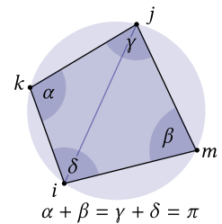
Fig. 22. There are many equivalent characterizations of the Delaunay triangulation. Here we illustrate a few examples.
