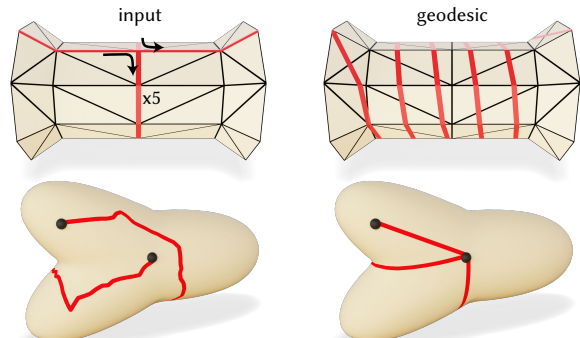
Fig. 36. Careful treatment of noncrossing curves enables finding geodesics that overlap many times ( top ), or those that get pulled tight around endpoints of the path itself ( bottom ).
