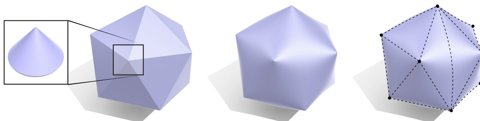
Fig. 12. Left : intrinsically, a small neighborhood around any vertex of a polyhedral surface is indistinguishable from a round circular cone. For instance, a vertex made from triangular pieces of paper can be easily smoothed out into a circular cone without stretching or ripping. Center : a good mental “cartoon” of an intrinsic triangulation is hence a surface where the edges are completely smooth, and only the vertices are visible. Right : from this perspective, no one triangulation is special—there are many intrinsic triangulations that describe the exact same geometry.
