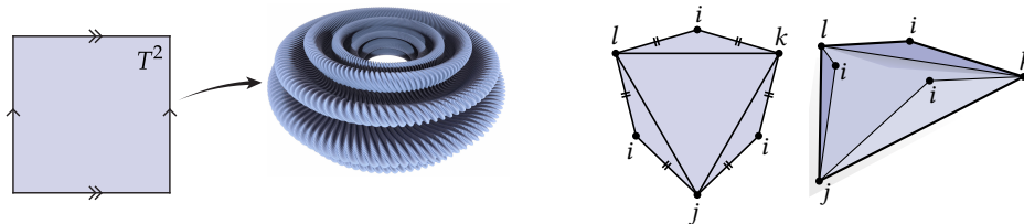
Fig. 10. Shapes that are difficult or impossible to embed in \mathbb{R}^n are often much easier to describe intrinsically. For instance, the flat torus (left) can be thought of intrinsically as a square with opposite edges identified—whereas finding a flat embedding into \mathbb{R}^3 is a major challenge (image from [Borrelli et al. 2013]). Likewise intrinsic triangulations that describe a perfectly reasonable metric space, such as the tetrahedron depicted in the right, may be impossible to embed into \mathbb{R}^3 while preserving lengths.
