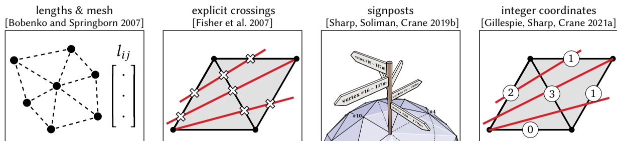
Fig. 18. The representations for intrinsic triangulations considered in this text.
