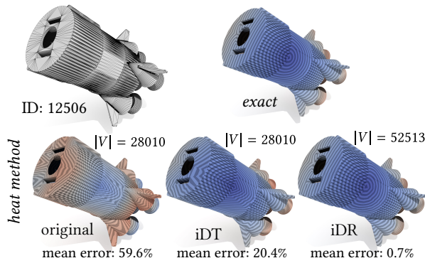
Fig. 29. Intrinsic triangulations dramatically improve the quality of solutions from PDE-based geometry processing algorithms such as the heat method when run on low-quality geometry. [Sharp et al. 2019b]
