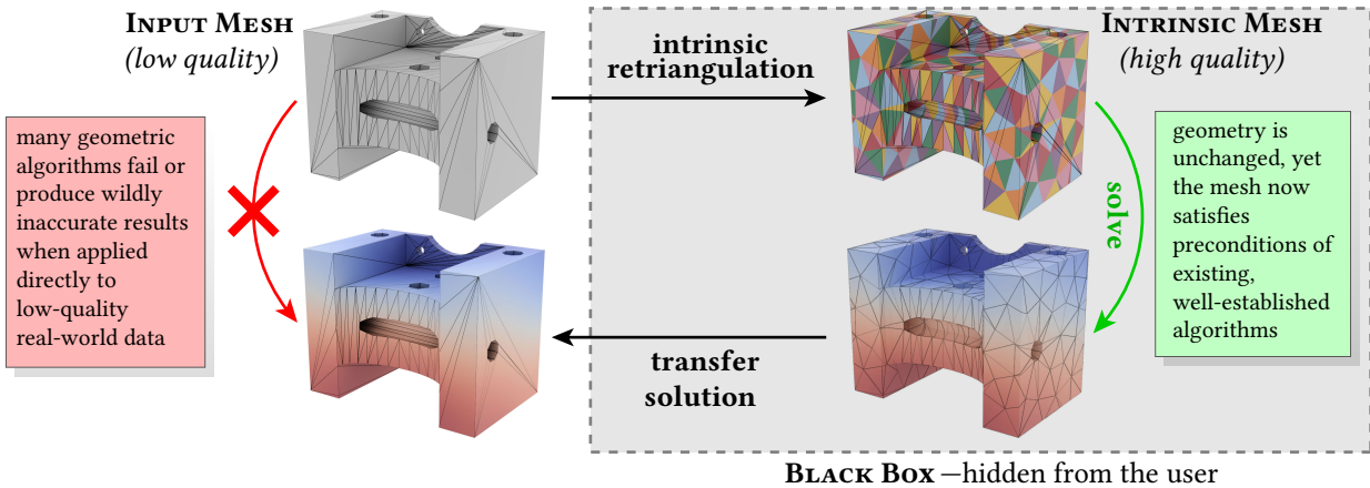
Fig. 1. There is a major gap between the kind of data expected by geometric algorithms, and the quality of data encountered in real applications. The high-level goal of this course is to build a bridge that allow existing algorithms to be applied in much more challenging scenarios. Here, a high-quality intrinsic triangulation is overlaid on top of a low-quality input mesh, enabling an existing finite element solver to compute a more accurate solution. Since the underlying geometry is completely unchanged, this solution can easily be transferred back to the original mesh for further processing—without the end user ever having to know that a transformation was applied “under the hood.”
