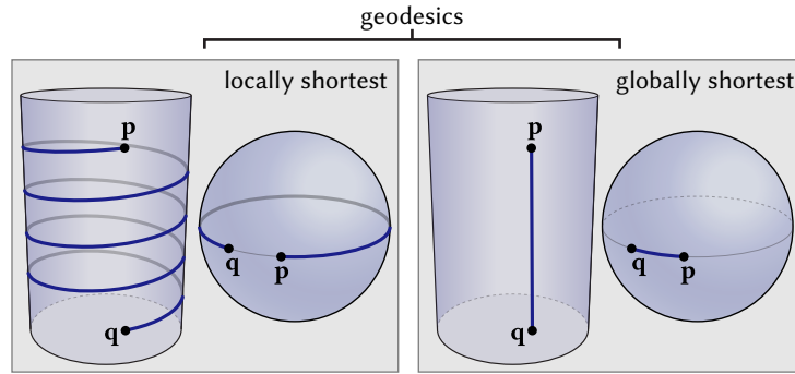
Fig. 15. A geodesic is often confused with a “shortest path” between points p and q , but in general a geodesic can be any path that locally minimizes length, or equivalently, that exhibits no tangential acceleration.
