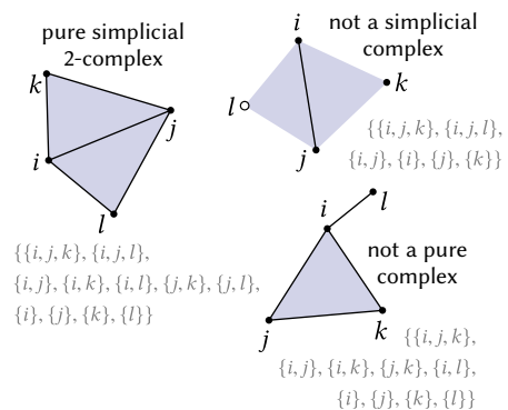
Fig. 5. In a simplicial complex, an edge must have two distinct endpoints, and a triangle must have three distinct vertices.
