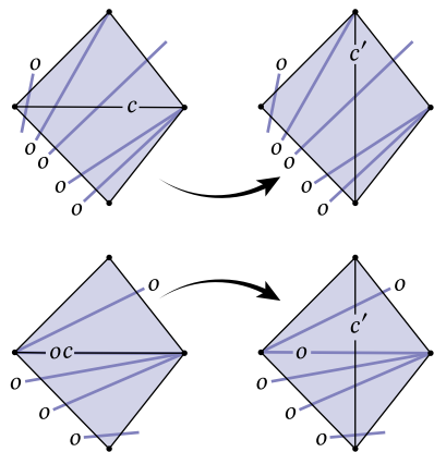
Fig. 19. Flipping an edge in the explicit crossing representation [Fisher et al. 2007].
