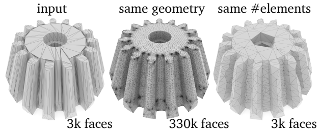
Fig. 27. Traditional remeshing cannot improve element quality without increasing mesh size or disturbing the geometry; intrinsic triangulations escape this tradeoff.
