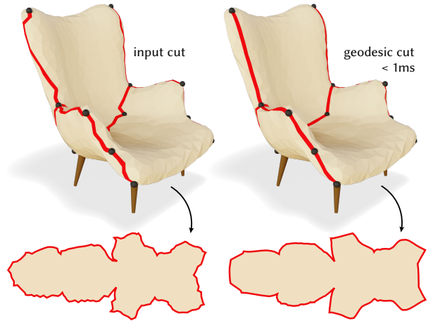
Fig. 39. Curve networks arise when cutting and flattening a shape for computational fabrication. Our method is perfectly suited to straighten an initial cut network along edges ( left ) to a geodesic network ( right ), yielding a much more natural pattern for fabrication ( bottom ).
