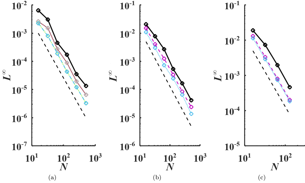
Figure 12: L^\infty norms of \Phi_e for various IBMs for a (a) circle, (b) 2D flower, and (c) sphere immersed boundary with Dirichlet IBC for a (a) parabolic and (b,c) trigonometric analytical solution. Black solid line: L; Red solid line: Q; Grey dotted line: QO; Blue dashed line: QGS; Green dotted line: QGSO; Blue dotted line: QIS; Purple dashed line: QISS1; Black dashed line: second-order convergence; N : number of cells in the x -axis.
