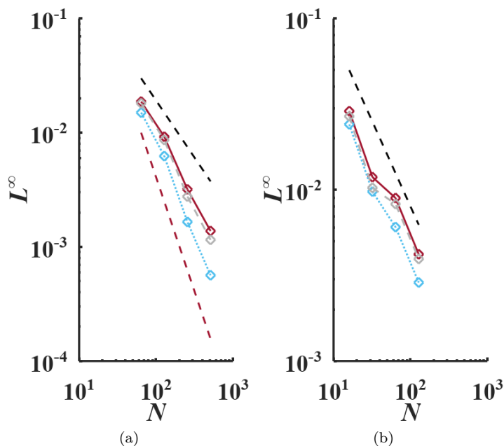
Figure 17: L^\infty norms of \Phi_e for various IBMs for a (a) circle and a (b) sphere immersed boundary with Neumann IBC and trigonometric analytical solution. Black solid line: L; Red solid line: Q; Blue dotted line: QGS; Grey dashed line: QIS; Black dashed line: first-order convergence; Red dashed line: second-order convergence; N : number of cells in the x -axis. The black and red solid line are superimposed on each other in (a) and (b).
