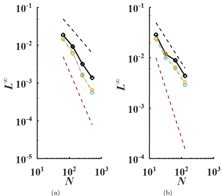
Figure 16: L^\infty norms of \Phi_e for various IBMs for a (a) circle and a (b) sphere immersed boundary with Neumann IBC and trigonometric analytical solution. Black solid line: L; Blue dashed line: LGS; Orange dotted line: LIS; Black dashed line: first-order convergence; Red dashed line: second order convergence; N : number of cells in the x -axis.
