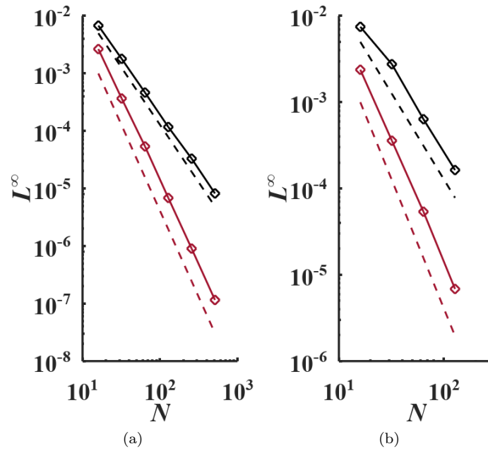
Figure 14: L^\infty norms of \Phi_e for a (a) circle and a (b) sphere immersed boundary with Dirichlet IBC and trigonometric analytical solution. Black line: p=2 ; Red line: p=3 ; Black dashed line: second order convergence; Red dashed line: third order convergence; N : number of cells in the x -axis.
