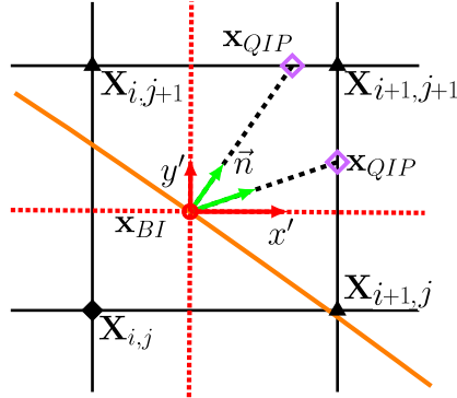
Figure 6: Close up view of possible quadrant intersection points \mathbf{x}_{QIP} for Q1 interpolation quadrant for a sample boundary intercept \mathbf{x}_{BI} . Solid orange line: \Gamma ; Dotted red line: Local axis (x', y') with origin at \mathbf{x}_{BI} ; Solid green vector: sample local surface unit normal to intersect line segments [\mathbf{X}_{i,j+1}, \mathbf{X}_{i+1,j+1}] and [\mathbf{X}_{i+1,j+1}, \mathbf{X}_{i+1,j}] ; Black diamond: ghost-cell; Black triangle: inner-cell.
