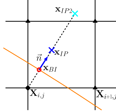
Figure 7: Close up view of the supplemental data points and values required for the quadratic methods for a sample ghost-cell \mathbf{X}_{i,j} . BI : Boundary intercept; IP : Image point; IP2 : Second image point; \vec{n} : local surface unit normal.
