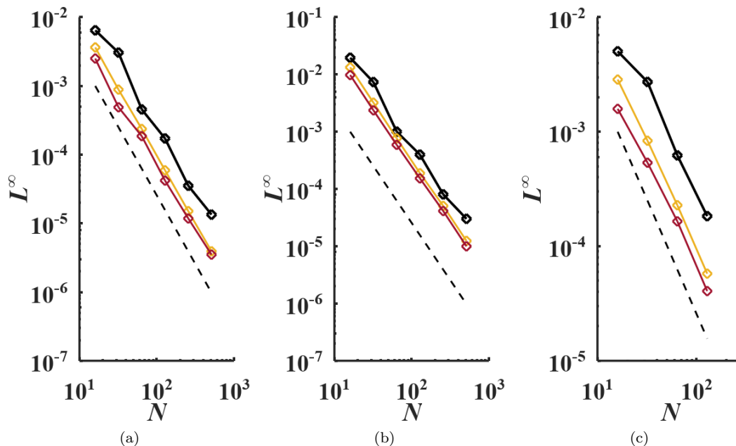
Figure 13: L^\infty norms of \Phi_e for various IBMs for a (a,b) circle and (c) sphere immersed boundary with Dirichlet IBC for (a,c) parabolic and (b) trigonometric analytical solution. Black solid line: L; Orange solid line: LGS with p=2 ; Red solid line: LGS with p=3 ; Black dashed line: second-order convergence; N : number of cells in the x -axis.
