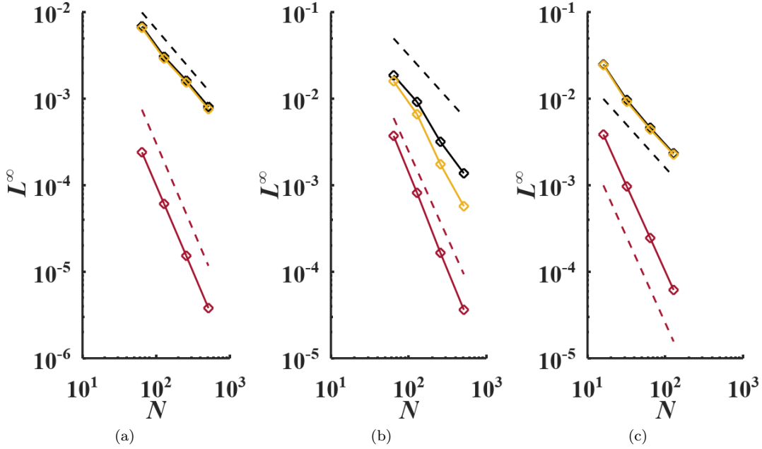
Figure 18: L^\infty norms of \Phi_e for various IBMs for a (a,b) circle and (c) sphere immersed boundary with Neumann IBC for (a,c) parabolic and (b) trigonometric analytical solution. Black solid line: L; Orange solid line: LGS with p=2 ; Red solid line: LGS with p=3 ; Black dashed line: first order convergence; Red dashed line: second-order convergence; N : number of cells in the x -axis.
