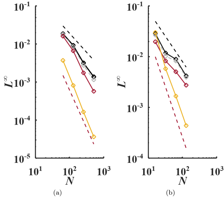
Figure 19: L^\infty norms of \Phi_e for a (a) circle and a (b) sphere immersed boundary with Neumann IBC and trigonometric analytical solution. Black line: L; Grey dotted line: QIS; Red line: QISS1 p=2 ; Orange line: QISS1 p=3 ; Black dashed line: first-order convergence; Red dashed line: second-order convergence; N : number of cells in the x -axis.
