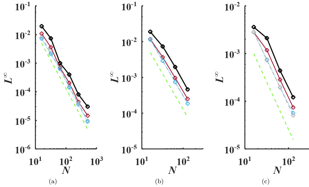
Figure 11: L^\infty norms of \Phi_e for various IBMs for a (a) circle, (b) sphere, and (c) 3D flower immersed boundary with Dirichlet IBC for a (a,b) trigonometric and (c) parabolic analytical solution. Black solid line: L; Red solid line: Q; Blue dotted line: QGS; Grey dashed line: QIS; Green dashed line: second-order convergence; N : number of cells in the x -axis. Blue dotted line and grey dashed line are superimposed on each other in (b) and (c).
