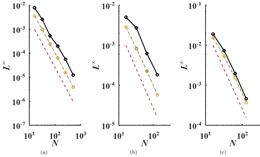
Figure 10: L^\infty norms of \Phi_e for various IBMs for a (a) 2D flower, (b) sphere, and (c) 3D flower immersed boundary with Dirichlet IBC for a (a,b) parabolic and (c) trigonometric analytical solution. Black solid line: L; Blue dashed line: LGS; Orange dotted line: LIS; Red dashed line: second-order convergence; N : number of cells in the x -axis.
