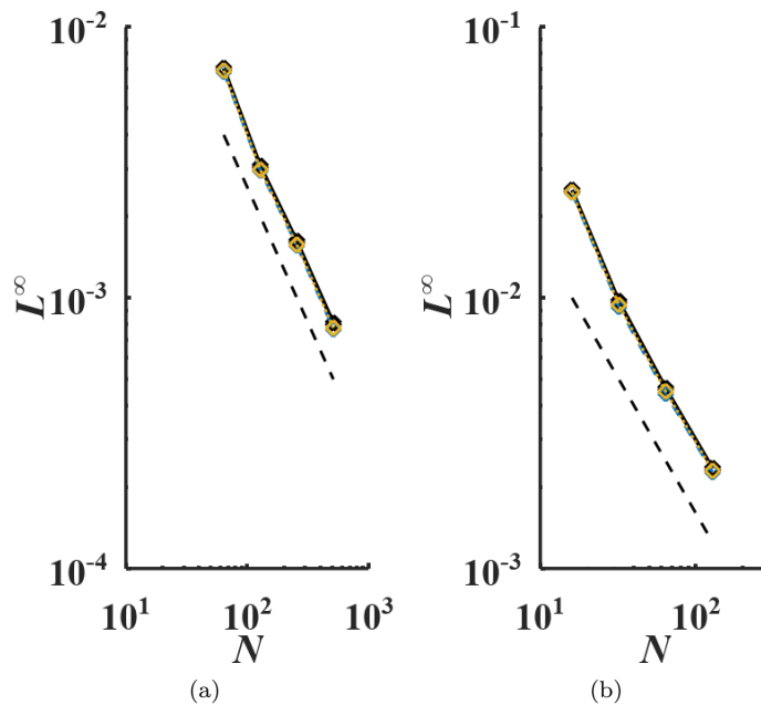
Figure 15: L^\infty norms of \Phi_e for various IBMs for a (a) circle and a (b) sphere immersed boundary with Neumann IBC. Black solid line: L; Blue dashed line: LGS; Orange dotted line: LIS; Black dashed line: first order convergence; N : number of cells in the x -axis.
