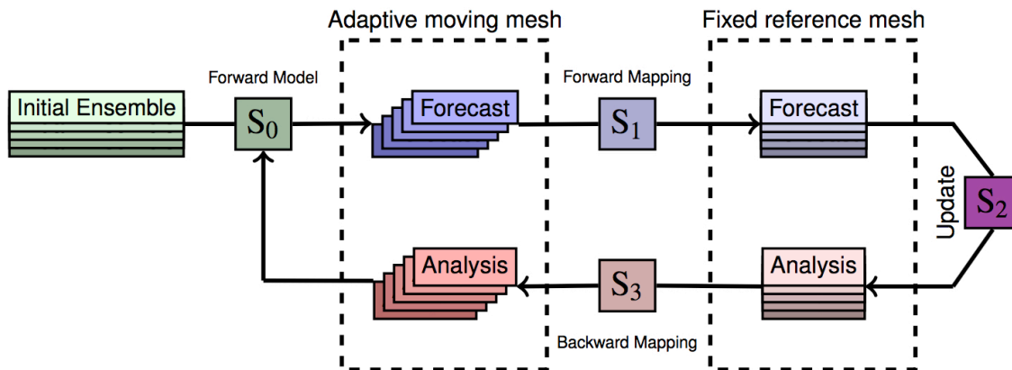
Figure 3. Illustration of the analysis cycle followed by in the proposed EnKF using method for adaptive moving mesh models. Each of In S_1 , adaptive moving meshes are mapped onto the processes S_0 , S_1 , S_2 and fixed reference mesh. The ensemble is updated on the fixed reference mesh at step S_2 (i.e. the analysis). Then, in S_3 the updated ensemble members are mapped back to the corresponding adaptive moving meshes. The full process is explained illustrated in Fig. 4 for one ensemble member. See text in Sect. 5 for full details on the individual process steps, S_0 , S_1 , S_2 and S_3 .
