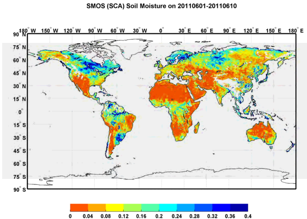
Figure 18a. Average estimated soil moisture using the single channel algorithm (SCA) for SMOS ascending orbits for the period of June 1-10, 2011.
