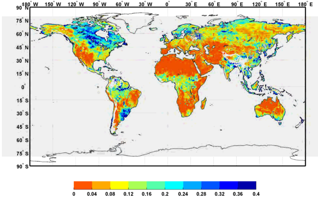
Figure 18b. Average estimated soil moisture using the single channel algorithm (SCA) for SMOS ascending orbits for the period of July 1-10, 2011.
