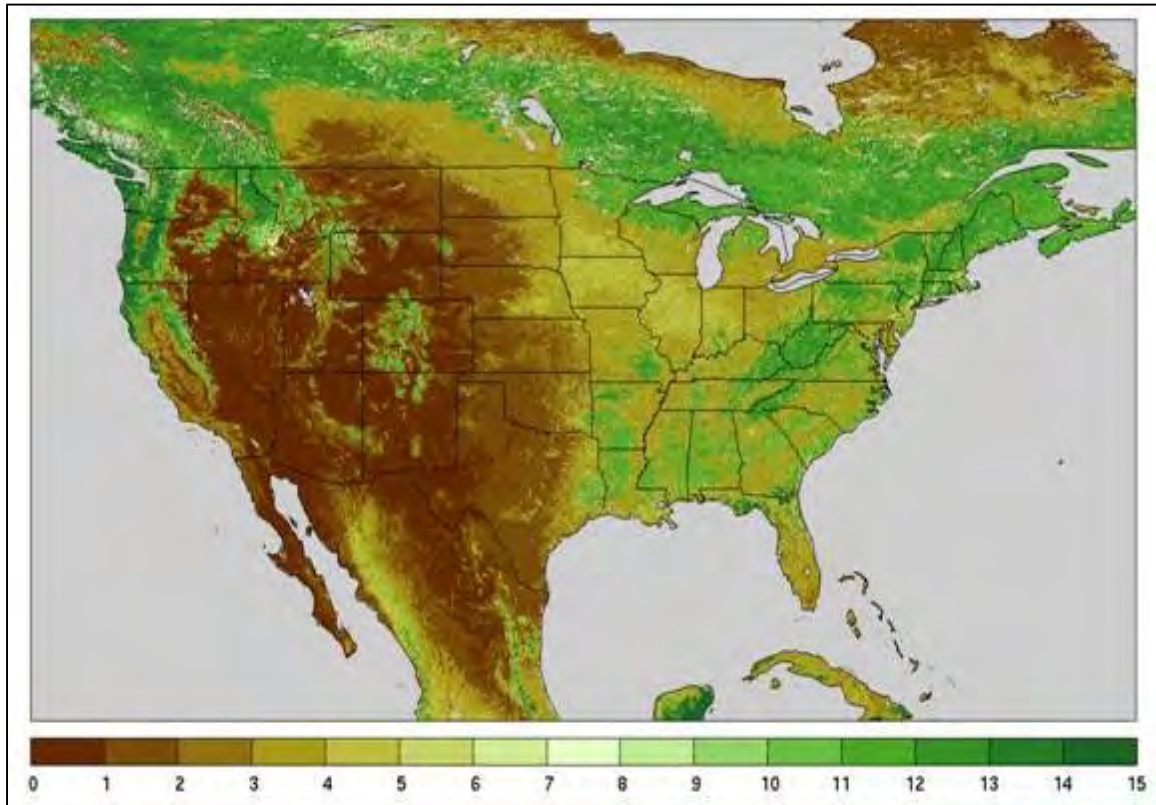
Figure 24. VWC over the continental U.S. for the month of July on a 1-km EASE grid as constructed from a 10-year MODIS NDVI climatology and land cover products. This new methodology for determining VWC was used in creating a new global 10-year MODIS NDVI climatology at 1 km spatial resolution for use by SMAP [41]. The new climatology was derived from MODIS data from 2000-2010, and is binned over 10-day periods throughout the year; prior to the SMAP launch, this climatology will be updated for the period 2000-2013. In the absence of concurrent NDVI data during the SMAP mission, the historical NDVI for any day of the year for any location can be determined and then used in the VWC calculation described in Equation 17; the annual maximum
