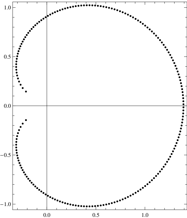
The 200 roots of P(200,x)
