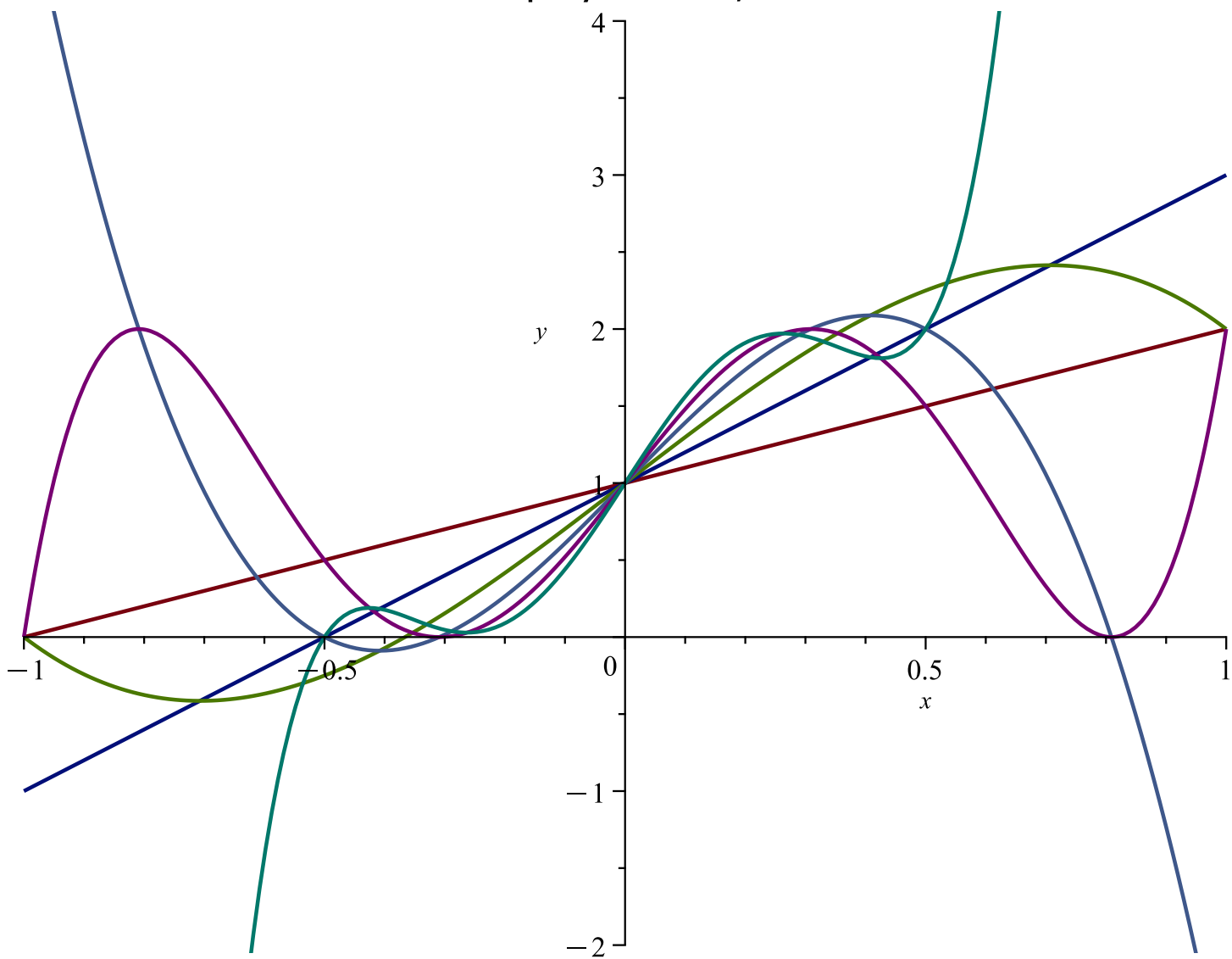
P363393 polynomials, n=1..6
