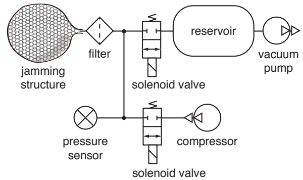
Figure 3: Pneumatic Jamming System. The system measures and controls the difference between atmospheric and internal volume pressure, such that particle jamming in the structure provides varying stiffness.
