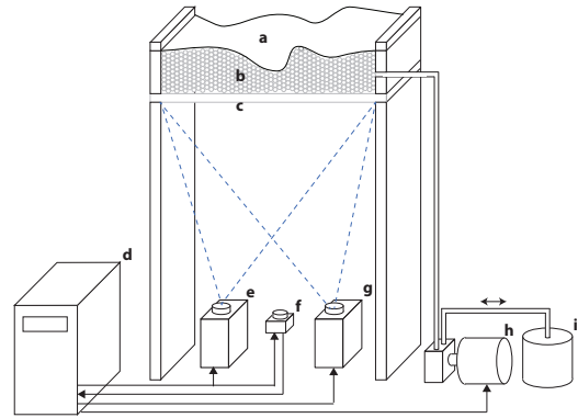
Figure 8: Structured Light Depth Sensing System with Index-Matched Jamming: (a) Silicone Membrane, (b) Pyrex glass beads and oil, (c) acrylic plate, (d) computer, (e) structured light IR projector, (f) IR camera, (g) graphics projector, (h) hydraulic pump, (i) reservoir
