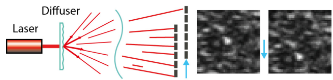
Figure 4: The speckle pattern motion can be tracked with image processing algorithms as the speckle sensor or projector move.
