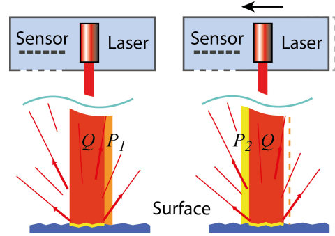
Figure 8: A device with an embedded speckle sensor and laser can detect its relative motion along a surface if the sensed inter-frame motion ( P_1-P_2 ) is significantly smaller than the laser beam's width. The speckles generated by the area Q will thus dominate the speckle pattern with frame-to-frame trackable patches.
