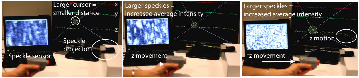
Figure 7: As the speckle sensor is moved closer to the speckle projector, speckles become larger in the image. While the speckle pattern is unknown, the statistically consistent distribution allows us to estimate distance with average intensity. Here, the distance controls the circle's radius in our software.
