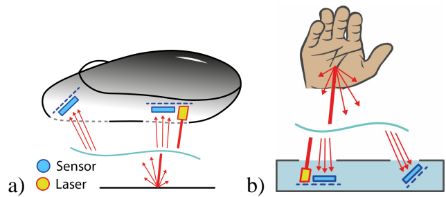
Figure 10: Hybrid tracking configuration F uses two speckle sensors to estimate relative motion orthogonal to a surface. a) Distance estimation with two embedded sensors in a mouse. b) The user's hand is used as a speckle generating surface when illuminated with collimated light, allowing its 3D motion to be tracked with two fixed speckle sensors.
