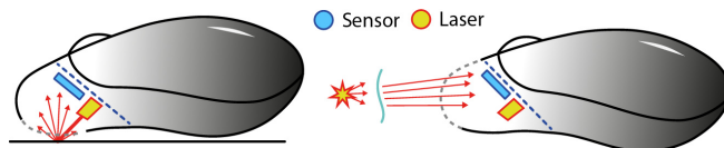
Figure 9: Hybrid tracking configuration E uses a speckle sensor at 45° to allow tracking both on the surface and in mid-air. An embedded laser creates speckle that can be sensed when the mouse is on the surface, while a speckle projector installed in the environment allows tracking in mid-air.
