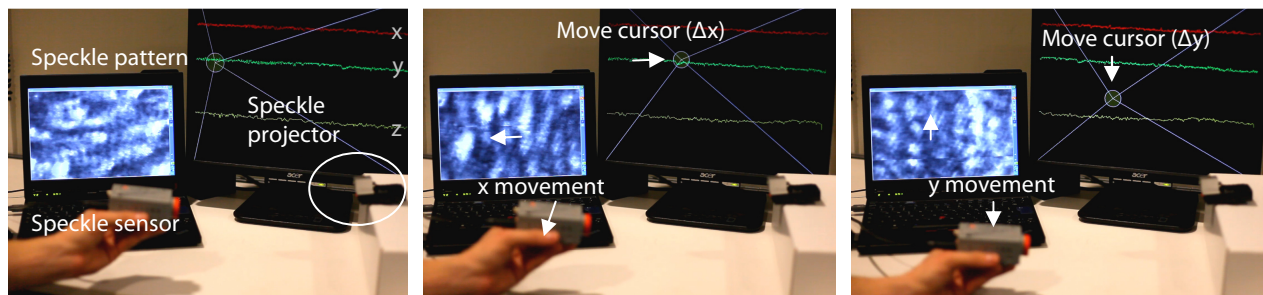
Figure 6: The speckle sensor is sensitive to small translations relative to the projected speckle pattern. A high frame-rate camera that is matched with the laser speckle characteristics can be used to track fine frame-to-frame movement. Here, the movement controls a cursor in our software.
