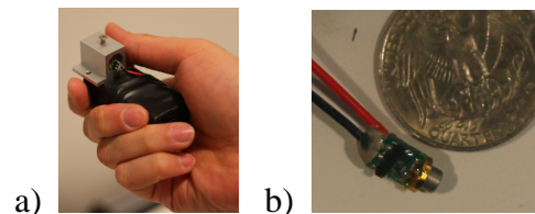
Figure 11. a) Our handheld Speckle Projector consists of a 50 mW laser (780 nm), diffuser (80°) and a battery. With our speckle sensors it has a 3 m range. b) The laser diode is only a few millimeters wide and could be integrated into various hardware configurations.
