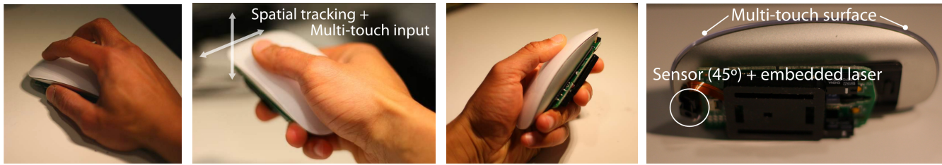
Figure 12: The TouchController works both as a regular mouse and in mid-air, tracked through a speckle projector in the environment. Its multi-touch surface enables a combination of spatial gestures and multi-touch interaction.
