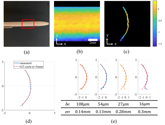
Figure 9. Reconstruction as a function of coherence length. (a) A natural image of the target, a cylindrical pen, marking the reconstructed region. (b) Depth reconstruction. (c) A side view of the reconstruction showing the circular curve. (d) The measured depth map fitted with the expected circular shape. The average error is around 0.1 mm. (e) We repeat the experiment multiple times under different coherence lengths \Delta c and, as expected, the error increases with decreasing \Delta c .
