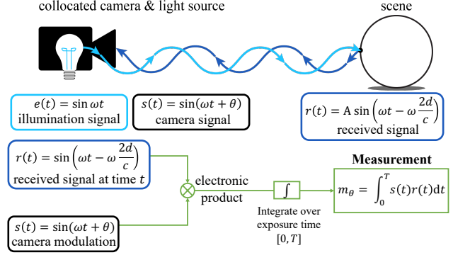
Figure 2. CW-ToF imaging systems. CW-ToF cameras use high-frequency illumination sources and exposure codes to indirectly measure the object’s depth. The measurement is the product of the delayed illumination signal and programmatically phase-shifted exposure code. The delay encodes object depth and is recoverable by taking multiple measurements with varying phase-shift ( \theta ).
