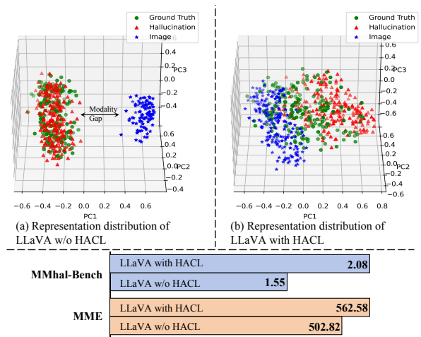
(c) The blue bar represents overall score on MMhal-Bench and the orange bar represents the overall score on MME. Noted bigger numbers mean better results.
