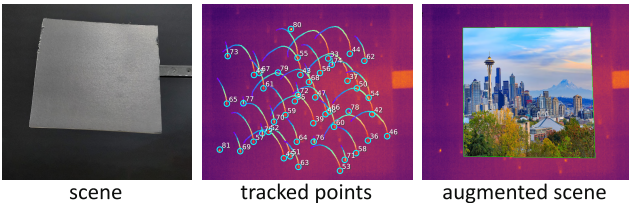
Figure 8. Augmented reality. Tracking the featureless plane’s 3D pose enables superimposing a picture on the plane’s surface.
