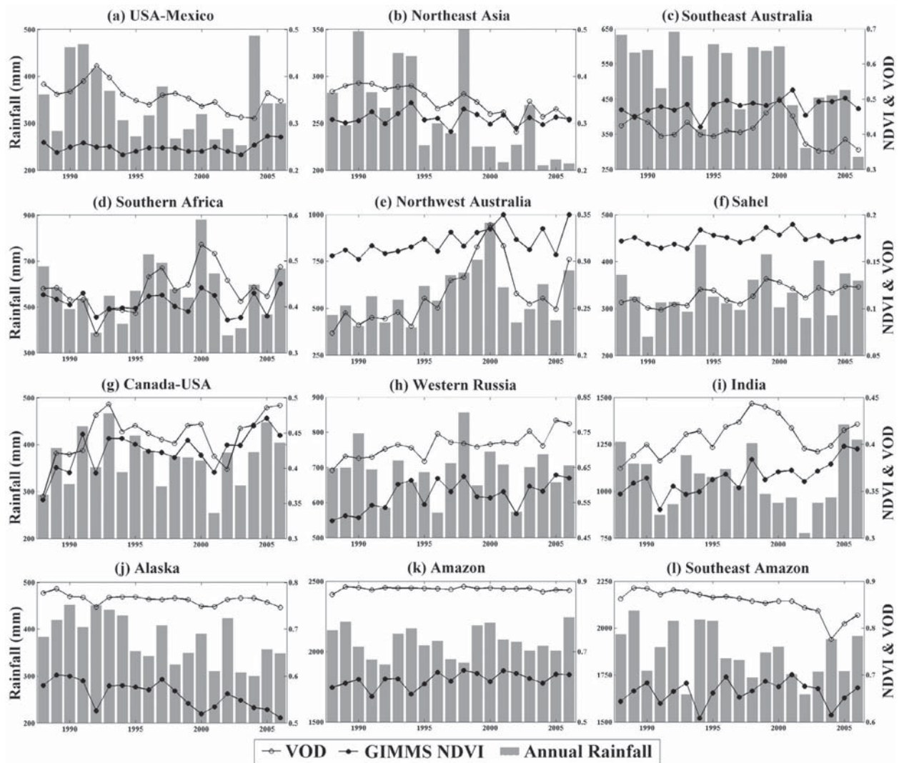
Figure 3. Annual average VOD, NDVI and total precipitation from 1988 through 2006 for the twelve regions outlined in Figure 2. Both VOD and NDVI are presented in their original values and share the right-hand y-axis. Note that vertical scales vary for visualization purpose.
