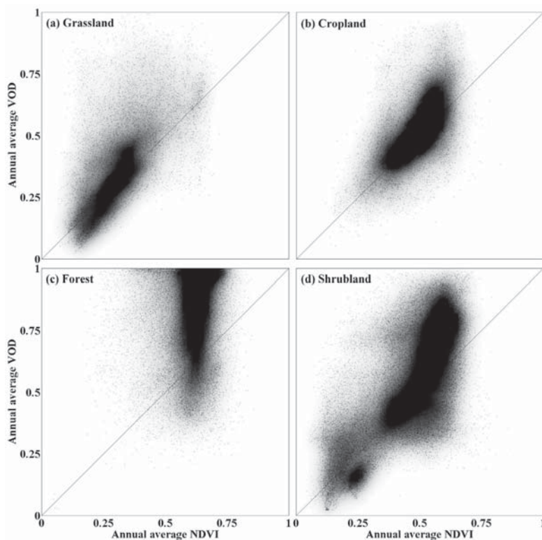
Figure 1. Relationship between annual average NDVI and VOD for 1987–2006 over different land cover types taken for each 0.25^\circ grid cell at the global scale. Here, the forest includes evergreen, deciduous, and mixed forests, while shrubland includes shrubland, woodland and wood/grass. Each scatter plot is overlain by a density plot; black, gray and white, respectively, representing high, medium and low density.
