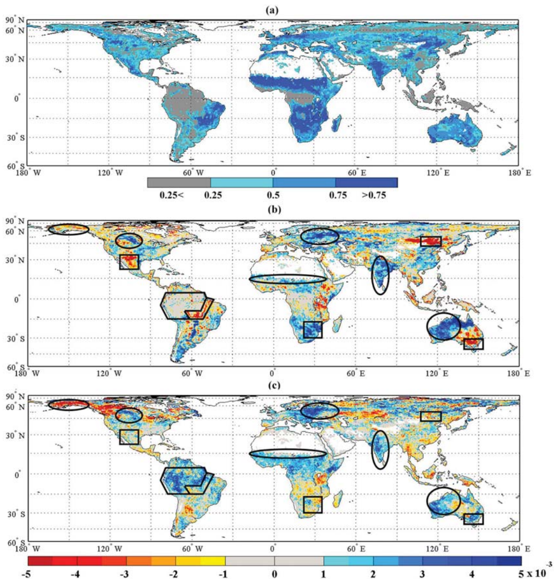
Figure 2. (a) Correlation coefficient ( r ) between monthly VOD and NDVI for 1987 through 2006; and trends in annual averages of (b) VOD and (c) NDVI from 1988 through 2006 (unit: change per year). The ranges of annual averages of VOD and NDVI (see Figure 1) are 0 to 1 and 0.1 to 0.8, respectively.
