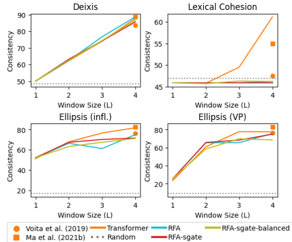
Figure 3: Model performance on the consistency test set, broken down into phenomena. Transformer and RFA are tested with window sizes from 1 to 4. We compare with the baselines in Voita et al. (2019) and Ma et al. (2021b) corresponding to our Transformer L = 4 .
