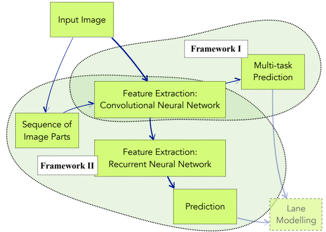
Figure 2. Diagram of Lane Recognition using Deep Neural Networks. This figure shows the workflow of the two frameworks for lane recognition proposed in this paper. Both frameworks employ convolutional neural networks for feature extraction. Framework I predicts both the presence of the targets and relevant geometric attributes. Framework II first process an input image as a sequence of regions of interest (ROI's), and applies two steps of feature extraction on each ROI: by convolutional neural networks and by recurrent neural networks. The latter can automatically recognise global structures over multiple ROIs. Optionally, higher level models (such as those in [6], [7], [8]) of the lane structures can be constructed based on the predictions. This step is shown as a transparent box "Lane Modelling". The details of the two frameworks are explained in Fig. 3 and Fig. 5, respectively.
