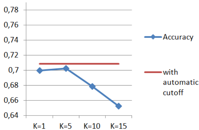
Fig. 9. Evaluation of the accuracy of the Cosine Similarity-based approach for finding relevant articles, using the class labels associated to the articles. Note that the accuracy levels reached by the automatic technique is higher than with the use of fixed cutoffs.
