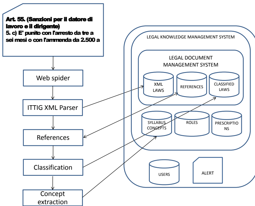
Fig. 1. Key components of the Eunomos system
