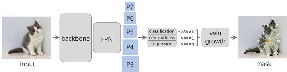
Figure 3: Overall architecture. H and W are the height and width of feature maps. k and n are the instance category number and the polar coordinate direction number. Vein growth is responsible for assembling masks. The ‘white circles’ are fixed contour points. The ‘black circles’ are generated dynamically according to instance shapes.
