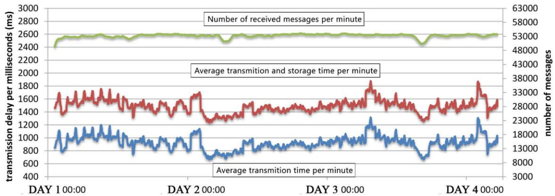
Fig. 4-14 Scalability test.
