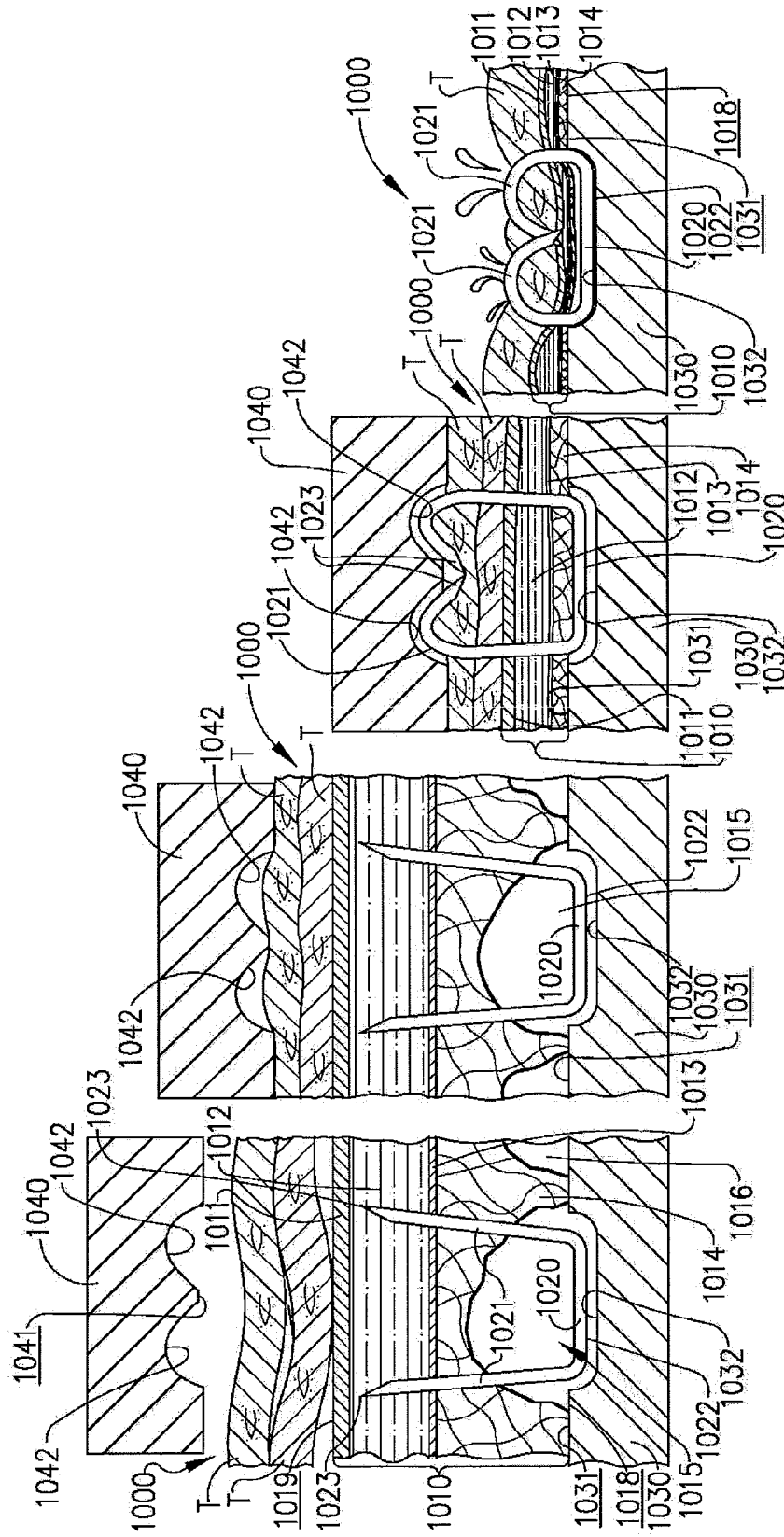
JAW OPEN FIG. 18A JAW CLOSED FIG. 18B STAPLES FORMING FIG. 18C COMPLETELY FORMED FIG. 18D
