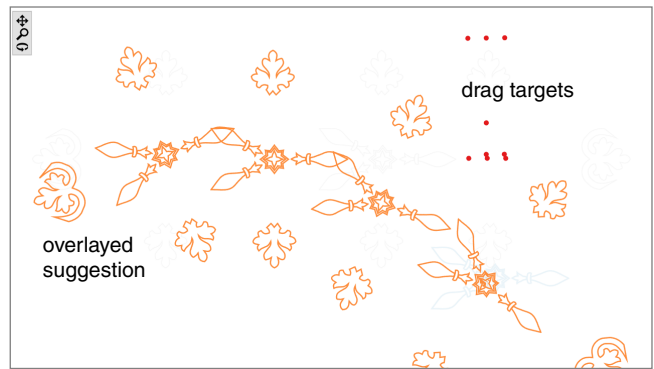
(b) Auto-complete
