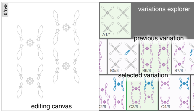
(a) Exploration
