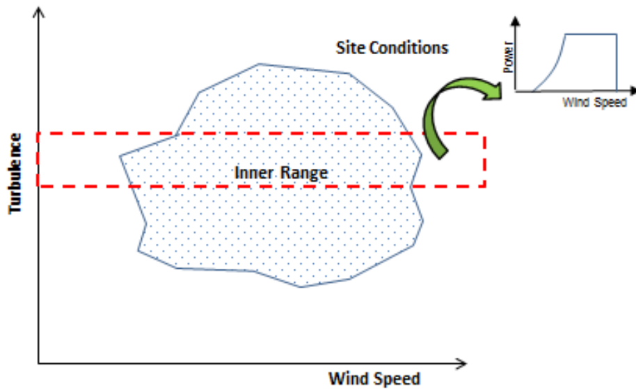
Figure A1. Illustration of the data analysis process used to extract an inner-range power curve from a participant dataset.
