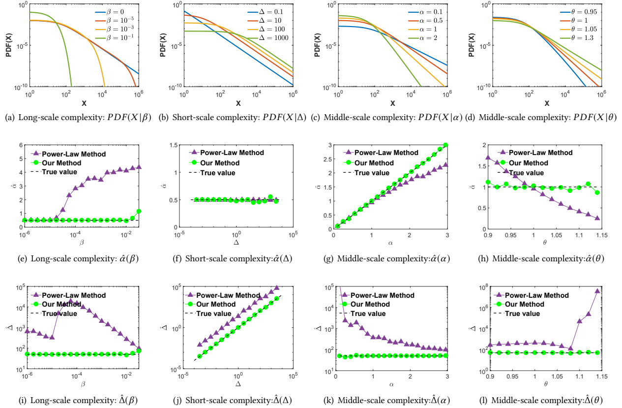
Figure 3: Complexities in short-, long-, and middle- scale regimes introduce systematic biases to the previous method. Our method fits reality well. The first row shows the distributions with different complexities in different regimes. Last two rows shown mean estimated values for the modeling parameters plotted as a function of the varying parameter which capture the complexity in corresponding regime. Figures in each column are of same settings. In all cases, the statistical errors are smaller than the data points. The true parameter values are shown in dashed lines. The pdf described in PL method is f(x) = \frac{\alpha_{PL}-1}{x_{min}} (\frac{x}{x_{min}})^{\alpha_{PL}} , where \alpha = \alpha_{PL} - 1
