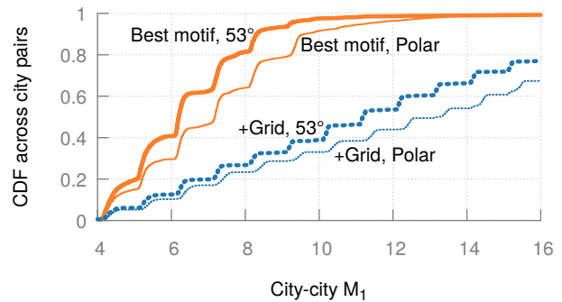
Figure 10: For the same constellation size, performance improves with inclined orbits as satellites spend less time over sparsely populated polar regions. Improvement over +Grid is similar for both constellations.
