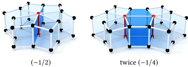
Fig. 4. (Left) Interior singular edge of valence 6 in red. Dark blue faces indicate the location of dual sheet insertion. (Right) Hex mesh after dual sheet insertion. The single valence 6 edge is split into two valence 5 edges.
