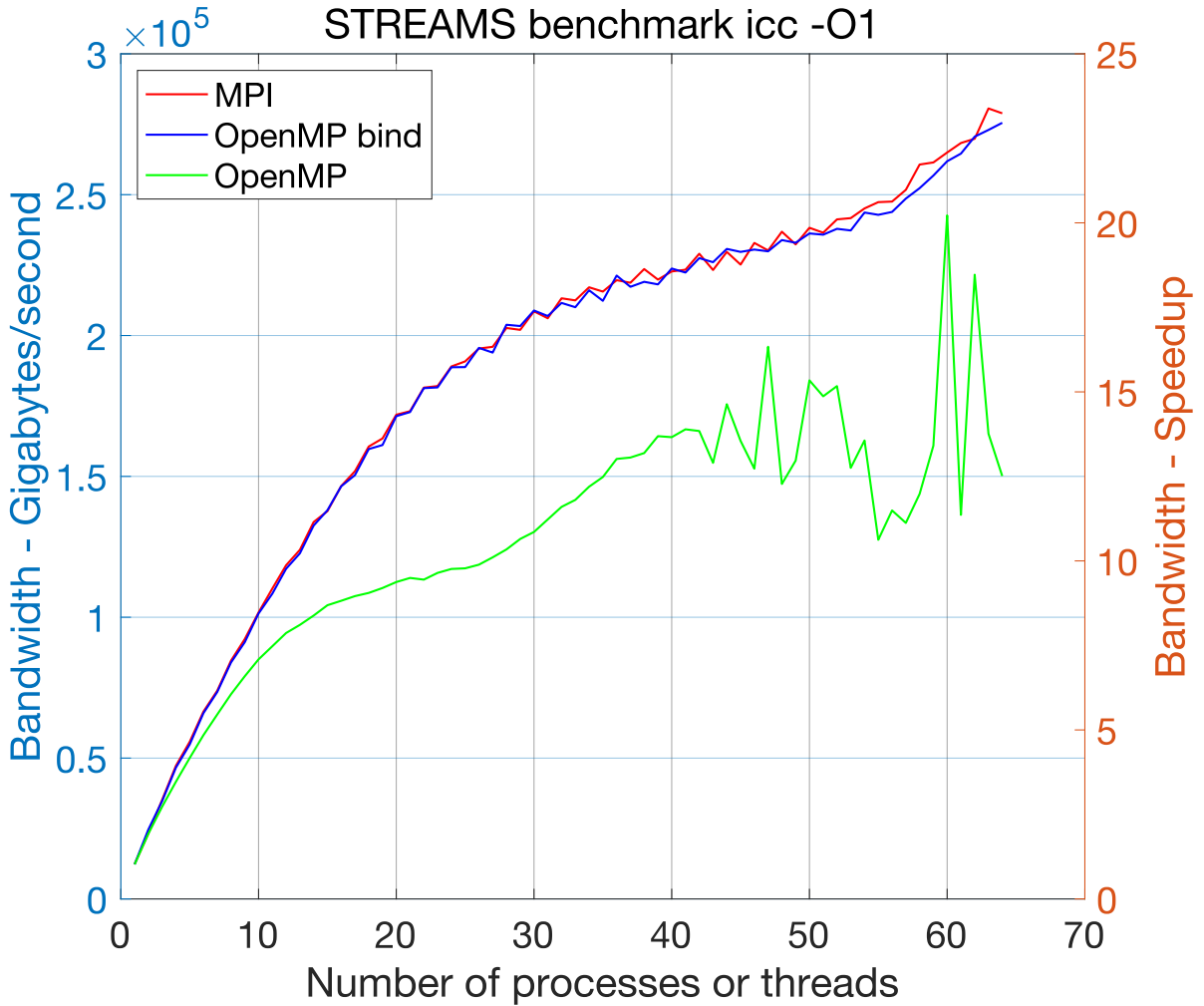
Fig. 4.8: STREAMS benchmark icc -O1
