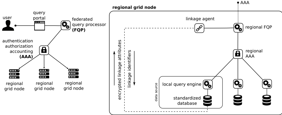
Fig. 1. Schematic for a distributed architecture for federated query processing.
