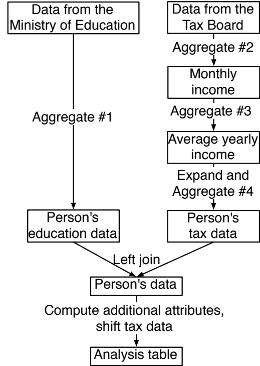
Fig. 2. The privacy-preserving ETL process of the study
