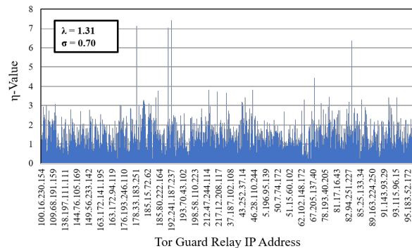
Fig. 4. Max-Divergence value across all possible Counter-RAPTOR Tor guard relays in the Top 93 Client ASes for the month of October 2017.
