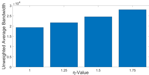
Fig. 30. Average bandwidth of guard relay choice for the Updated DPSselect algorithm for different \eta -values.
