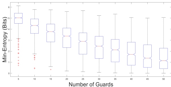
Fig. 2. Distribution of Min-Entropy of Counter-RAPTOR clients in AS5432 client AS over multiple guard observations in 1000 different simulations.
