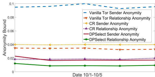
Fig. 17. MATor Anonymity Bound 10/1/2017 - 10/5/2017
