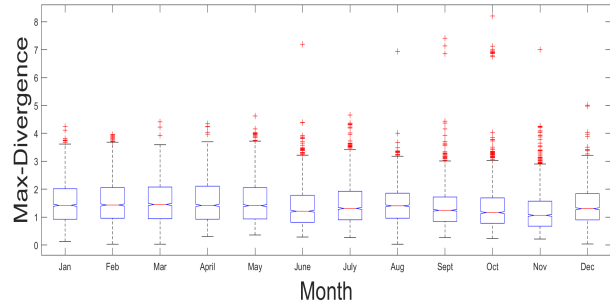
Fig. 6. Distribution of the Max-Divergence ratio across actives Tor guards in each month of 2017.
