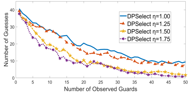
Fig. 27. \eta -value vs Minimum Guessing entropy of DPSselect after multiple guard relay selections in 100 simulations for clients in AS5432.
