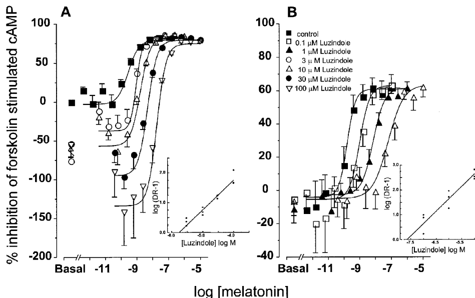
Figure 6 Antagonism by luzindole of melatonin-induced inhibition of forskolin-stimulated cyclic AMP production in CHO- mt_1 (A) and CHO- MT_2 (B) cells. Data are mean \pm s.e. mean of 3–4 separate experiments. Inset: Schild plots depicting antagonism of melatonin responses by luzindole. The line through the data was plotted using the parameters obtained from the analysis described in the Methods.
