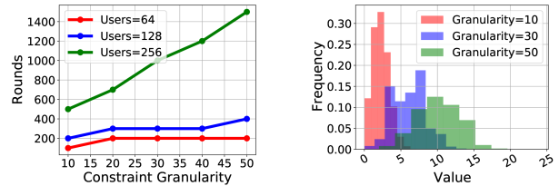
(a) Rounds required to reconstruct P with 100% accuracy vs constraint granularity. (b) Histogram of number of user participations across constraint windows.
