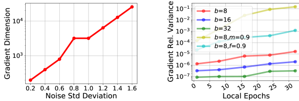
(a) Number of parameters of the gradient dimension required to recover P exactly. (b) Relative noise of FedAvg updates on Cifar10 LeNet; batch size b , momentum m , dataset fraction f .
