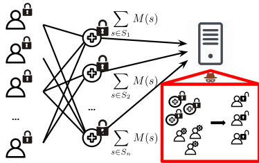
Figure 1. Our gradient disaggregation attack observes multiple rounds of aggregated model updates and leverages side channel information in the form of summary analytics collected by federated learning systems (how often users participated across certain training rounds) to uncover individual users’ private model updates, undermining the secure aggregation protocol. Code: https://github.com/gdisag/gradient_disaggregation .
