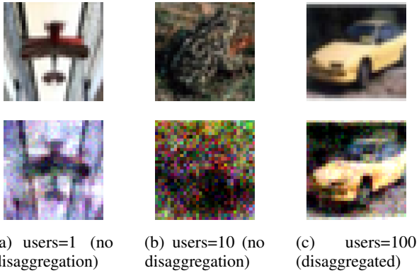
Figure 8. Recovered images from FedAvg updates across users (top image is closest ground truth). Gradient disaggregation enables high quality inversion on noisy FedAvg updates aggregated across many users; unlike disaggregation on exact gradients, disaggregation on noisy updates recovers the average update submitted across rounds, and we are able to reconstruct high quality images on noisy updates aggregated across many users. Without disaggregation, inversion on updates aggregated over multiple users (users=10) significantly degrades quality.
