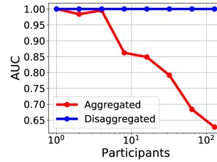
Figure 9. Property inference with and without gradient disaggregation (main task: gender classification, auxiliary task: identifying images of specific race) on FedAvg updates. Gradient disaggregation enables property inference on individual model updates and maintains high AUC score across increased number of users.
