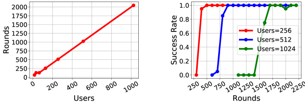
(a) Rounds required to reconstruct P with 100% accuracy vs number of users. (b) Success rate of recovering columns of P versus rounds.
