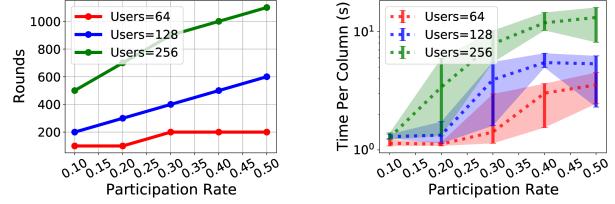
(a) Rounds required to reconstruct P with 100% accuracy vs participation rate. (b) Mean, min, and max runtime to reconstruct columns of P vs participation rate.
