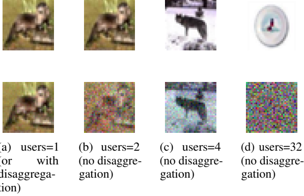
Figure 7. Recovered images from gradients across users (top image is the closest ground truth). Gradient disaggregation recovers individual users’ exact gradients, hence, performing the gradient inversion attack with gradient disaggregation on multiple users yields the same quality as performing the attack on just one user. Without disaggregation, gradient inversion fails on gradients aggregated across more users.
