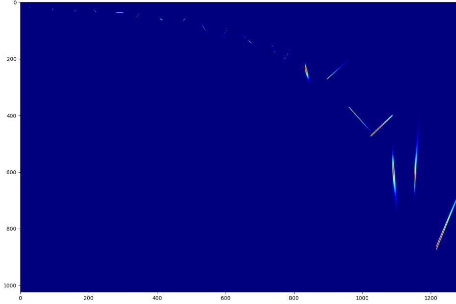
Figure 7: Bird: This dataset proposes to predict the presence or absence of a bird in short audio clips. A priori, detection of such events heavily relies on chirps, the characteristic sound of birds with increasing/decreasing frequency over time. We can see from the learned filters how the learned representation indeed focuses on such patterns, reach super-resolution and thus extreme sensitivity to the time and frequency position of the events, in particular for medium to low frequency kernels. For high frequency kernels, the time and frequency resolution is further increased.
