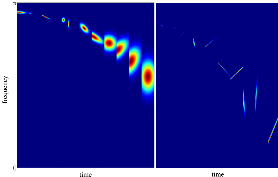
Figure 4: Depiction of the learned filters \Psi[., f] (Def. 1). The full filters banks can be found in Appendix B, the vertical over horizontal axes ratio is 1. Left, our learned representation on AudioMNIST dataset (Becker et al., 2018) : This noiseless speech pushes the filters with high frequency resolution (easily seen from the filter covariance as per (6)). For some of these filters the time resolution is also very high (reaching super-resolution), while others favor local translation invariance. For all the medium to low frequency filters, great frequency and time invariance is preferred with large gaussian support, with a slight chirpiness for the medium frequency filters. Thus, the low frequency filters tend to favor time resolution. Right, our learned representation on Birdvox dataset (Lostanlen et al., 2018) : We see that the detection of bird songs heavily relies on chirps. Indeed the characteristic sound of birds is increasing or decreasing in frequency over time. Moreover, the learned representation demonstrate filters that reach super-resolution. Thus it encodes with high precision the time and/or frequency position of the events per Prop. 2) as the cost of being more sensitive to input deformation. It fits with the extreme time-frequency accuracy of bird audition and acoustic production (Dooling and Lohr, 2006).
