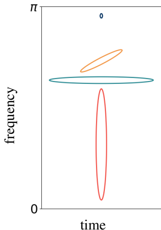
Figure 1: Visualization of four different Gaussian filters \Phi in the time-frequency plane (the Wigner-Ville domain) each depicted with a different color. Interpretability of the filters (as detailed in Sec. 3.2) can be done directly by looking at the mean (position) of the Gaussian and the covariance matrix. In this case, the black/top filter is highly localized in time and frequency near the Nyquist frequency (notice the much higher localization than allowed in a WT or STFT; the orange/anisotropic filter is encoding chirp events (linear change in time of the instantaneous frequency), this is typical of bats or birds’ calls; the green/flat filter is highly localized in frequency and encodes long duration event, this can be seen with insects emitting relatively high frequency sounds for a long duration; the red/bottom filter on the contrary is localized in time and encodes large band frequency events, this is typical of transient events such as clicks of dolphins.
