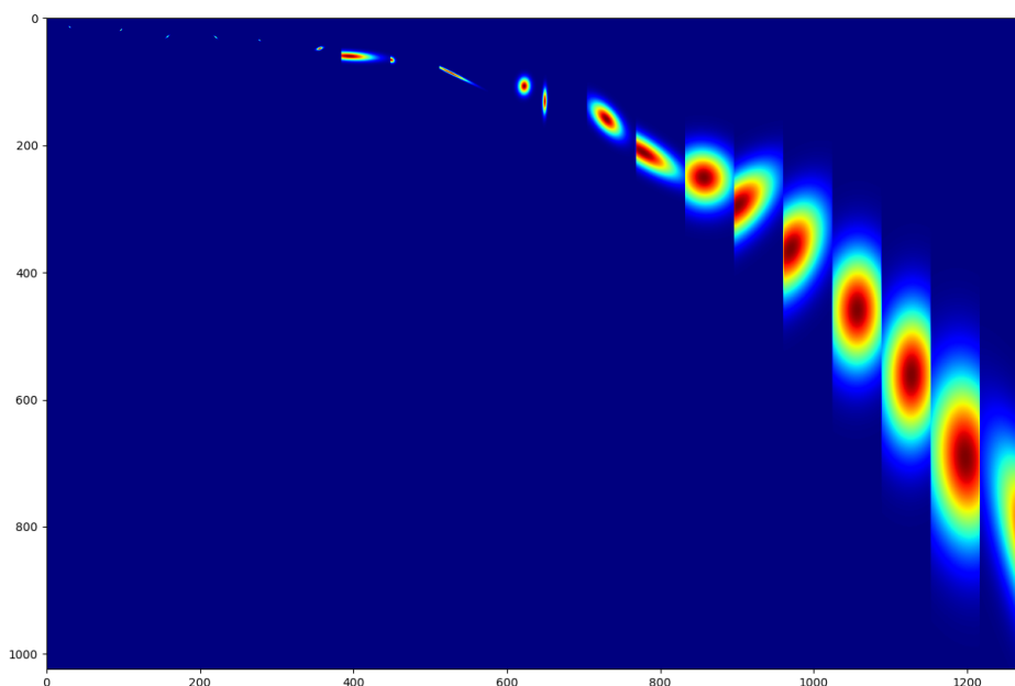
Figure 5: Audio MNIST: this dataset deals with spoken digit classification. A few key observations: the high frequency filters tend to take an horizontal shape greatly favoring frequency resolution, for some of the filters the time resolution is also very high (reaching super-resolution) while others favor local translation invariance. For all the medium to low frequency filters, great frequency and time invariance is preferred (large gaussian support) with a slight chirpiness for the medium frequency filters. The low frequency filters tend to favor time resolution.
