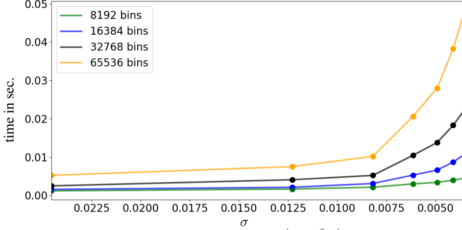
Figure 3: Computation time (in sec.) to evaluate \text{WV}_x \star \mathcal{N}(\cdot; \mathbf{0}, \sigma^2 I_2) on signals x of different lengths depicted with different colors and with varying \sigma . The smaller \sigma the more localized in time and frequency is the representation, in the limit case of \sigma \rightarrow 0 the produced representation falls back to the WV transform. An increase in the length of the signal x incurs a linear increase in computation time. The outer left case has similar computation time than the corresponding STFT with same \sigma for its frequency bandwidth.
