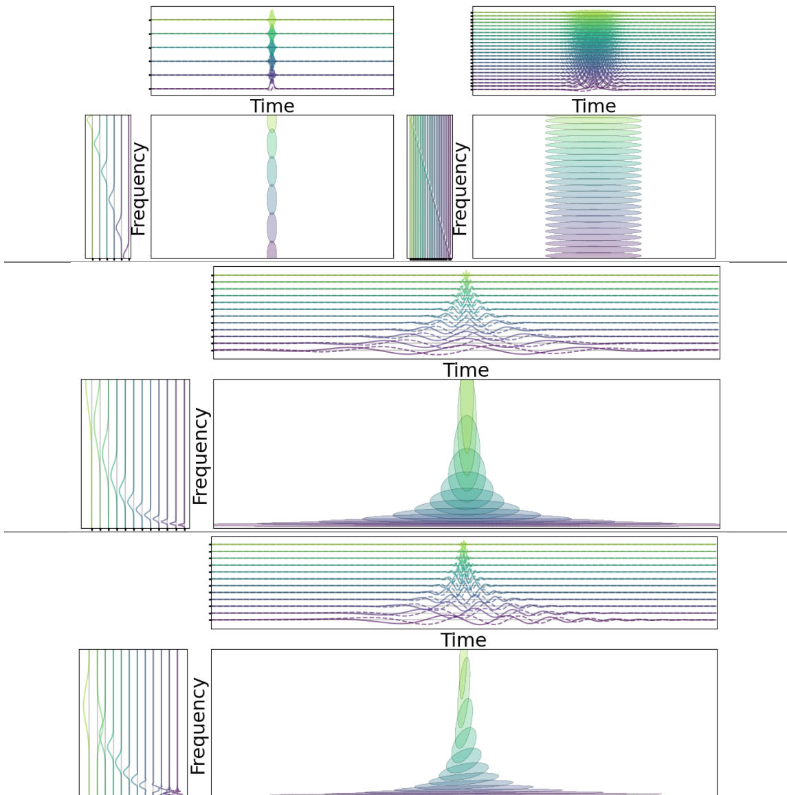
Figure 2: Depiction of various filter-banks in the frequency domain, time domain and time-frequency plane (Wigner-Ville domain) for a STFT ( top ) with small Gaussian apodization window (left) and large Gaussian apodization window (right); for a wavelet transform ( middle ) with Morlet wavelets, and for a chirplet transform ( bottom ). First, all those TFRs can be obtained through a Gaussian filtering of the Wigner-Ville representation each with a specific set of means and covariances for the Gaussians. By changing those parameters it is possible to move continuously from one TFR to another (Theorem 1). Second, the larger is the Gaussian (covariance) in one direction or the other (time or frequency) the more stable will be the produced TFR (Prop. 2), with an highly localized Gaussian (small covariance entries) super-resolution is achieved providing the produced TFR increased time and/or frequency precision of the events present in the input signal. Third, learnability of the Gaussian parameters allow to let the data, classification/regression pipeline and the loss function at hand drive the design of the TFR to maximize performances.
