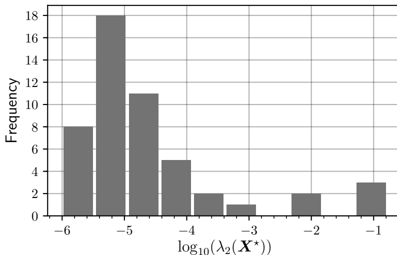
Figure 1: SDP primal spectrum for small n . We plot a histogram of the second-largest eigenvalue of X^* the optimizer of \text{SDP}(\mathbf{W}) , over 50 trials with n = 150 .
