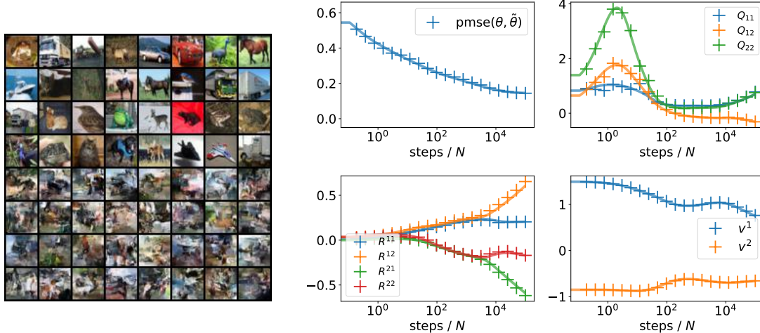
Figure 4: Theory vs experiments for online SGD with deep, pre-trained realNVP model of Dinh et al. (2017). (Left) The top four rows show images drawn randomly from the CIFAR10 data set, the bottom four rows show images drawn randomly from the realNVP model trained on CIFAR10. (Right) Same plot as Fig. 2 when inputs are drawn from the pre-trained realNVP. D = N = 3072 . In all experiments: M = K = 2 , \tilde{v}^m = 1 , \eta = 0.2 , g(x) = \tilde{g}(x) = \text{erf}(x/\sqrt{2}) , integration time step dt = 0.01 .
