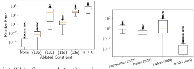
(a) This figure plots the relative error when constraints in (14) are ablated. While removing (13b) typically results in reasonable relaxation gaps, the removal of any relaxations. The 0-SOS relaxation, (14), as well as other constraint renders the relaxation entirely uninformative with gaps typically on the order of 10^2 . (b) This figure shows the relative relaxation gap of the SOS relaxation, (14), as well as those of several existing gaps. The removal of any relaxations. The 0-SOS relaxation is often exact, with relaxation entirely uninformative with gaps typically of magnitude smaller than the other relaxations.
