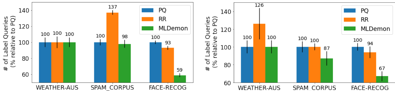
(a) Lower monitoring risk: \eta=0.15 . The baseline avg. query rate for PQ is 7.4% on WEATHER-AUS, 7.1% on SPAM-CORPUS, and 1.3% on FACE-RECOG.
