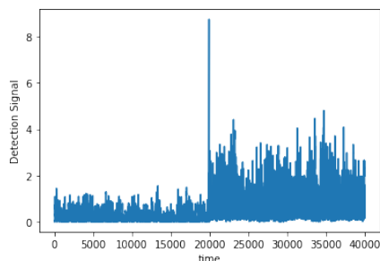
(e) Detection signal G_t
