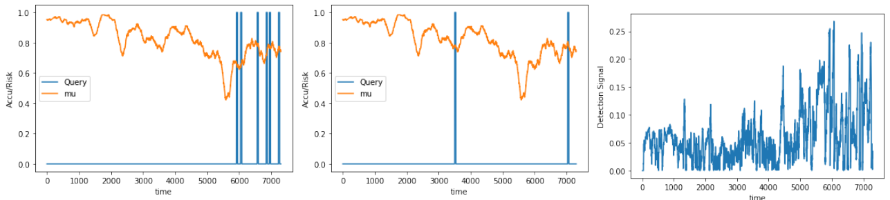
(a) RR at \phi=0.2 . RR queries for 6 batches at empirical risk R=886.6 .
