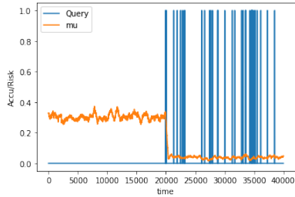
(b) RR at \phi=3 .
