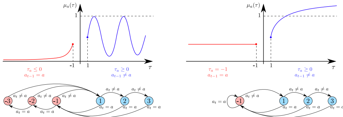
Figure 1: Transition mechanisms (reduced to 6 and 4 states), and examples of expected reward function \mu_a for LSD Bandits (left) and models with delay-dependent rewards (Kleinberg and Immorlica, 2018, e.g.) (right).
