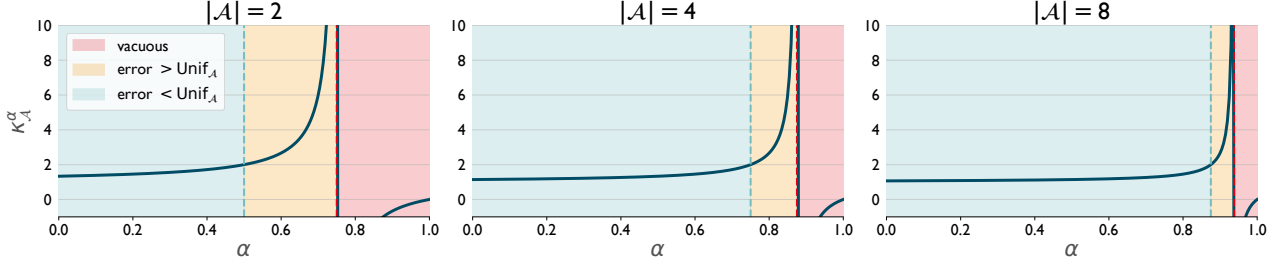
Figure 4.1: As |\mathcal{A}| grows, regularizing using \pi_0 with larger d_{\text{TV}}(\pi^*(\cdot|s), \pi_0(\cdot|s)) will converge to a lower error than log-barrier regularization. In other words, there is a more forgiving margin of error for the default policy.
