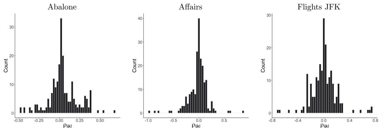
Figure 3: Histogram of \rho_{i,j,k,l} \equiv \text{Cov}((h_i(X) - h_j(X))(h_k(X) - h_l(X))) for the Abalone, Affairs and Flights JFK datasets.
