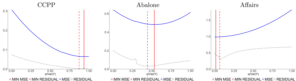
Figure 2: Plots of normalized values of \text{MSE}(q) and \text{RES}(q) for three different datasets. The solid and dashed vertical lines correspond to the value of \hat{g}_2 that minimizes the MSE and residual curves respectively.
