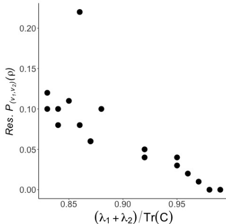
Figure 4: Normalised residual norm \mathcal{P}_{(v_1, v_2)}(\rho) vs (\lambda_1 + \lambda_2)/Tr(\hat{C}) , of the various manually crafted ensembles for the 17 datasets.
