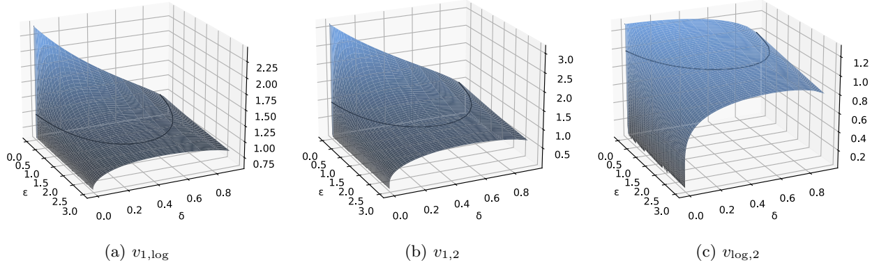
Figure 1: For pairs of Logistic(log), Laplace (1), and Gaussian (2) distributions: plots of variance ratios v_{a,b} and contours where the resulting variances are equal.
