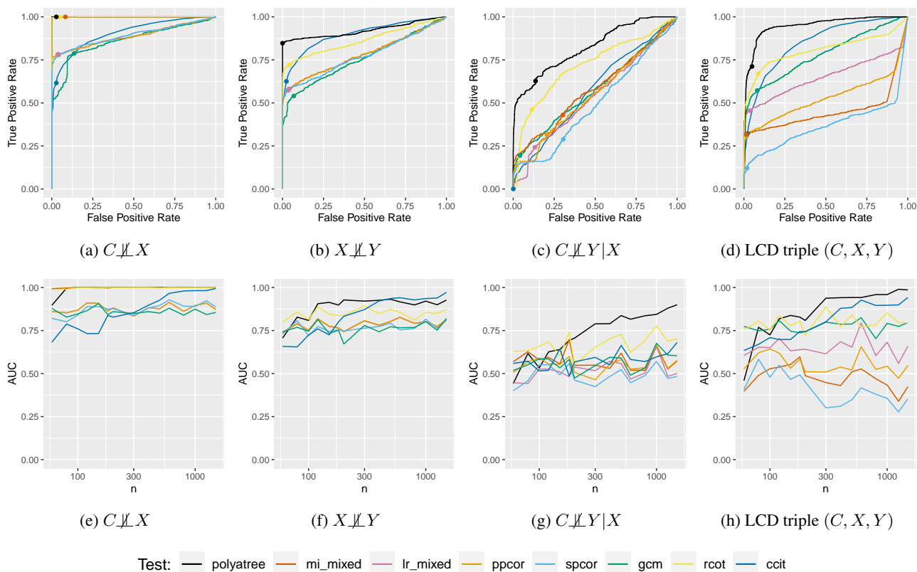
Figure 4: ROC and AUC results for simulated data. The first row depicts ROC curves for individual tests (a–c) and for the LCD algorithm (d) over 2000 rounds of simulations at sample size n = 400 . The second row depicts the median AUC for varying sample size (ranging from 60 to 1500) for individual tests (e–g) and for the LCD algorithm (h) over 200 rounds of simulations.
