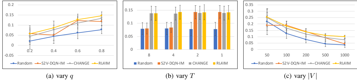
Figure 5: Performance of different methods on unseen test graphs. The x-axis is the value of the underlying setting, and the y-axis is the expected normalized influence (w.r.t. the number of nodes) averaged over 10 \times 20 = 200 runs.
