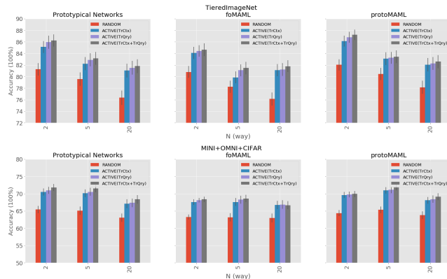
Figure 2: Comparison of random selection (RANDOM) and active selection (ACTIVE) during meta-train for the composition of the query set (TrQry), context set (TrCtx) and their combination (TrCtx+TrQry) for varying N when the episode sizes T are N \times 10 on TieredImageNet and MINI+OMNI+CIFAR.
