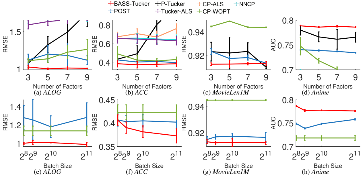
Figure 1: Predictive performance with different numbers of factors (top row) and streaming batch sizes (bottom row). In the top row, the streaming bath size is fixed to 512; in the bottom row, the factor number is fixed to 5. The results are averaged over 5 runs. Note that the performance of several baselines are missing or incomplete, because they are far worse than all the other methods and hence not included.
