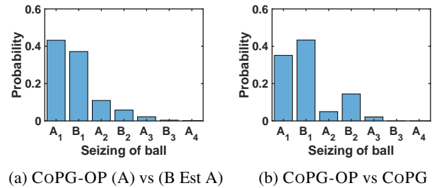
Figure 7: Interaction plots evaluated by playing 5000 games. Matches played between a) CoPG-OP player A and player B estimated by A b) CoPG-OP and CoPG
