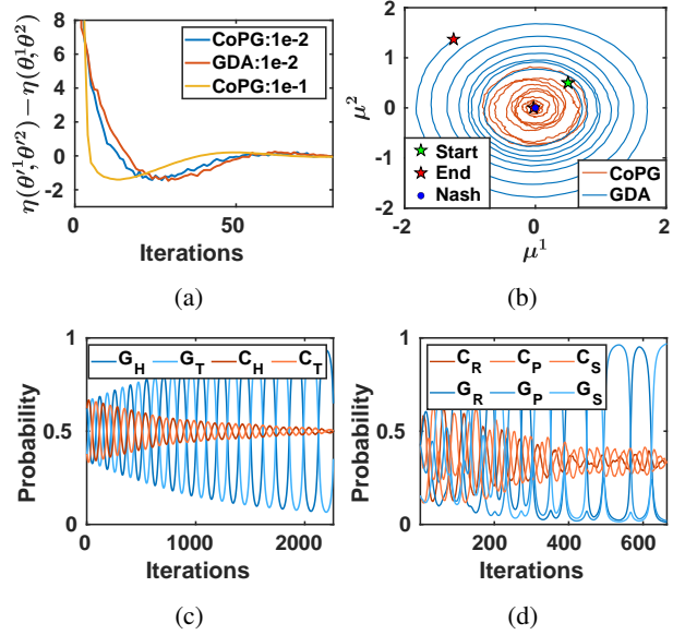
Figure 2: During training CoPG (C) vs GDA (G) on a) LQ game, difference in game objective due to policy update for \alpha = 1e - 1, 1e - 2 b) Bilinear game, \mu^1 vs \mu^2 c) MP, probability of selecting Head(H) and Tail(T) d) RPS, probability of selecting rock(R), paper(P) and scissors(S).
