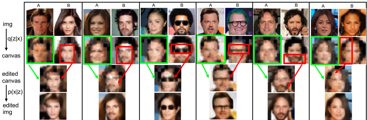
Figure 6: Latent space editing. Given images A and B, we encode them to obtain the latent canvases. Then we compose a new canvas by placing a portion of canvas B on top of canvas A. Finally, we decode an image using the composed canvas.
