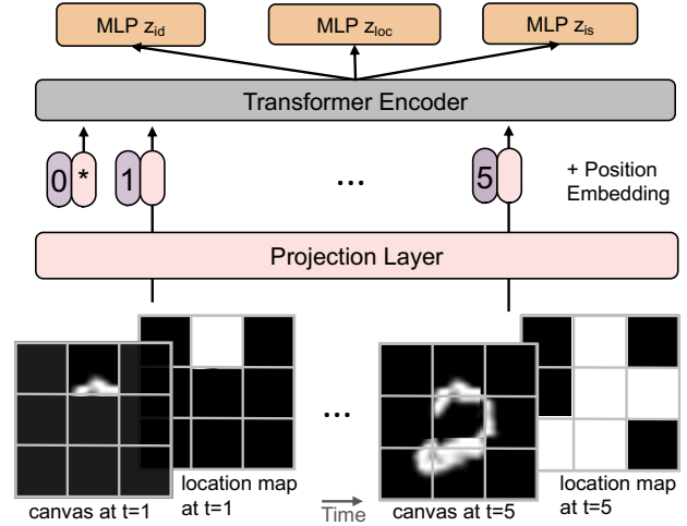
Figure 2: The Transformer-based conditional probability in Eq. (2). The input is a sequence of 2-channel images containing the canvas and the location map.
