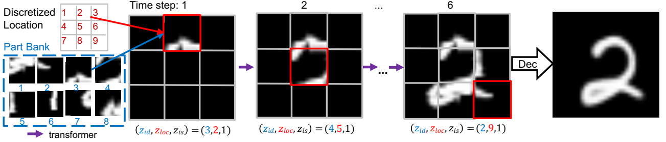
Figure 1: The generative process of our model. At each time step, a Transformer-based auto-regressive prior generates latent variables including what-to-draw \mathbf{z}_{id} (choosing a part from the part bank), where-to-draw \mathbf{z}_{loc} (choosing one of the discretized locations), and whether-to-draw \mathbf{z}_{is} (whether skipping the current step). The sampled image is generated from the final canvas via a decoder.
