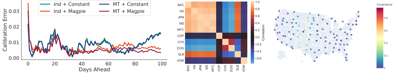
Figure 6. Left panel: Calibration error of both Volt and MT Volt at the 95% confidence level as a function of time step lookahead over 30 stocks from an entire sector ETF (XLF). While both are well-calibrated, MT Volt preserves well-calibration to longer time steps. Center panel: Estimated correlation matrix of stocks from two different sectors. MT-Volt successfully learns the high volatility correlation amongst the finance sector stocks (first five) with lower correlations between the energy sector stocks (second five). Right panel: Estimated volatility covariance with Boulder, CO. Correlations decrease as the stations go further away.
