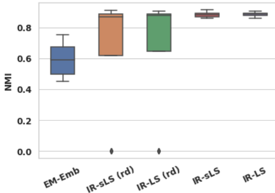
Figure 11: Average performance over 20 runs of our algorithms under the experimental setting of Section 5.1. Here (rd) indicates random initialization.
