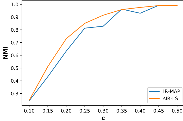
Figure 10: Average performance measured by NMI obtained with random initialization over 20 runs.
