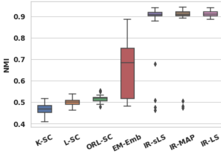
Figure 9: Performance of different algorithms on CSBM. Results are sorted by mean NMI and obtained over 40 runs.
