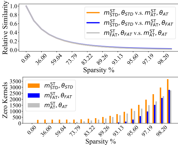
Figure A8. The statistic of subnetworks drawn from three different pre-training, i.e. (m_{STD}^{ST}, \theta_{STD}) , (m_{FAT}^{ST}, \theta_{FAT}) and (m_{AT}^{ST}, \theta_{AT}) . (Top): The relative mask similarity between subnetworks from different pre-training. (Bottom): The number of completely pruned (zero) kernels in these subnetworks.
