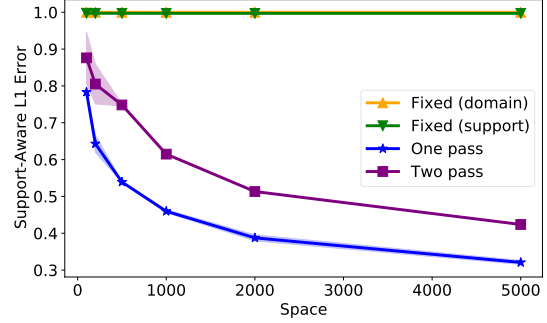
Figure 3. Comparison of support-aware L_1 error with varying space usage with k = 5 on the CAIDA dataset. Shading indicates one standard deviation over 10 trials.
