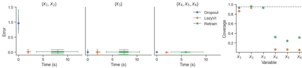
Figure 8. Distribution of computation time vs. estimation error relative to retrain ( \hat{v}_i - \hat{v}_i^{(RT)} ) for three different groups of variables: important, correlated ( \{X_1, X_2\} ); important, uncorrelated ( X_3 ); and unimportant, uncorrelated ( \{X_4, X_5, X_6\} ). 2D box plots show quantiles across 10 repetitions.
