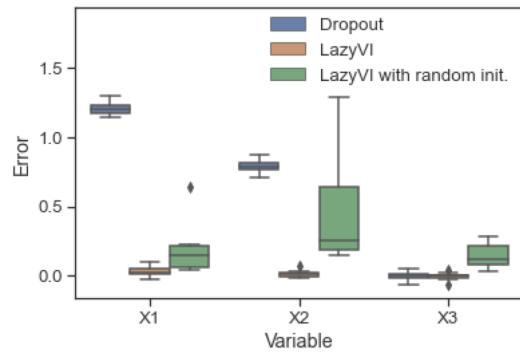
Figure 9. Distribution of VI - \hat{VI} for the first 3 variables for dropout, LazyVI initialized with the parameters from the full model, and LazyVI with a random initialization.
