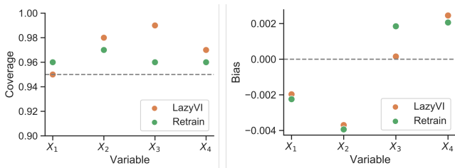
Figure 2. Left: Average coverage of empirical 95% confidence intervals from the LazyVI and retrain estimates across 100 simulations. Right: Average empirical bias (\hat{VI} - \hat{VI}) of LazyVI and retrain estimates.
