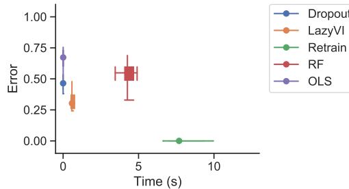
Figure 3. Distribution of computation time vs. normalized estimation error relative to retrain for the VI of X_1 ((\hat{VI} - \hat{VI}^{(RT)}) / \hat{VI}^{(RT)}) across 10 repetitions.
